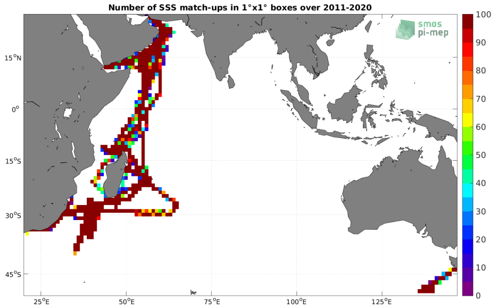
Figure 4: Number of SSS match-ups between TSG (GOSUD-Research-vessel) SSS and the SMOS SSS L4 v2 - Daily (BEC) SSS product for the Indian Ocean Pi-MEP region over 1^{\circ} \times 1^{\circ} boxes and for the full satellite product period.
