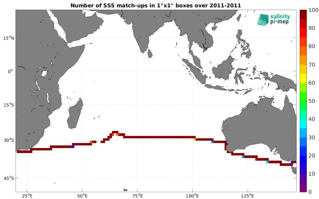
Figure 5: Number of SSS match-ups between TSG (CSIC-UTM) SSS and the SMOS SSS L4 v2 - Daily (BEC) SSS product for the Indian Ocean Pi-MEP region over 1^\circ \times 1^\circ boxes and for the full satellite product period.
