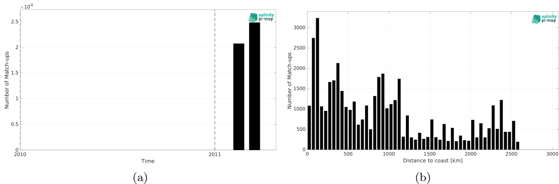
Figure 2: Number of match-ups between TSG (CSIC-UTM) and SMOS SSS L4 v2 - Daily (BEC) SSS as a function of time (a) and as function of the distance to coast (b) over the Indian Ocean Pi-MEP region and for the full satellite product period.
