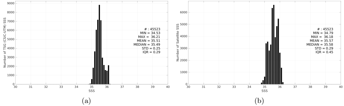
Figure 3: Histograms of SSS from TSG (CSIC-UTM) (a) and SMOS SSS L4 v2 - Daily (BEC) (b) considering all match-up pairs per bins of 0.1 over the Indian Ocean Pi-MEP region and for the full satellite product period.
