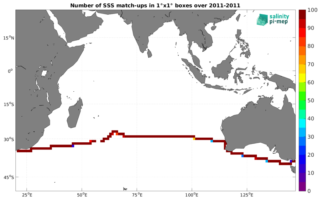
Figure 4: Number of SSS match-ups between TSG (CSIC-UTM) SSS and the SMOS SSS L4 v2 - Daily (BEC) SSS product for the Indian Ocean Pi-MEP region over 1^\circ \times 1^\circ boxes and for the full satellite product period.
