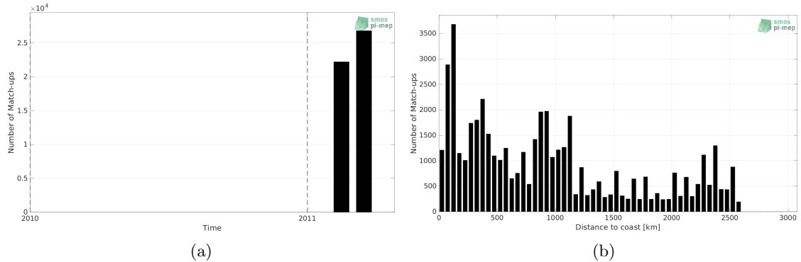
Figure 1: Number of match-ups between TSG (CSIC-UTM) and SMOS SSS L4 v2 - Daily (BEC) SSS as a function of time (a) and as function of the distance to coast (b) over the Indian Ocean Pi-MEP region and for the full satellite product period.
