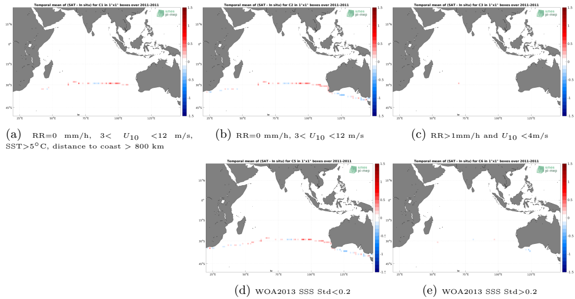
Figure 12: Temporal mean gridded over spatial boxes of size 1^\circ \times 1^\circ of \Delta SSS (SMOS SSS L4 v2 - Daily (BEC) - TSG (CSIC-UTM)) for 5 different subdatasets corresponding to:RR=0 mm/h, 3 < U_{10} < 12 m/s, SST >5^\circ C, distance to coast > 800 km (a), RR=0 mm/h, 3 < U_{10} < 12 m/s (b), RR >1 mm/h and U_{10} < 4 m/s (c), WOA2013 SSS Std <0.2 (d), WOA2013 SSS Std >0.2 (e).
