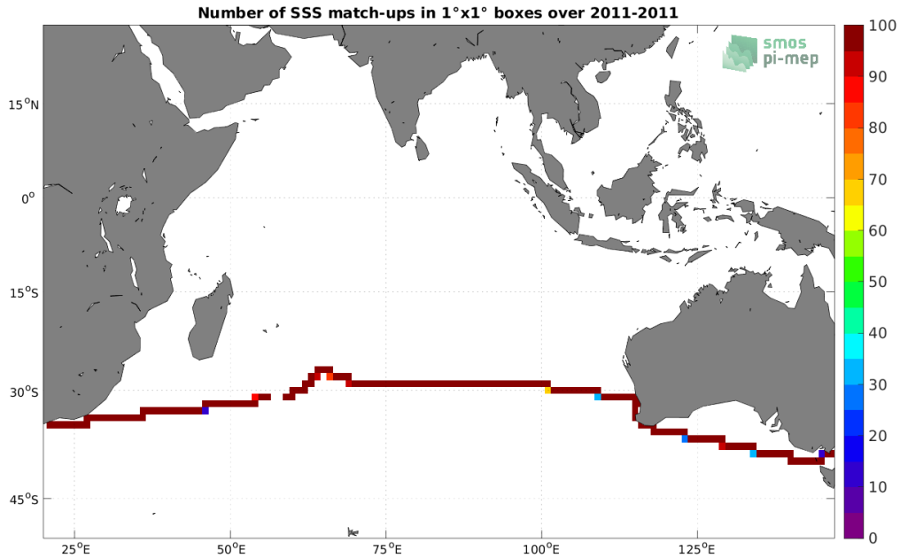
Figure 4: Number of SSS match-ups between TSG (CSIC-UTM) SSS and the SMOS SSS L4 v2 - Daily (BEC) SSS product for the Indian Ocean Pi-MEP region over 1^\circ \times 1^\circ boxes and for the full satellite product period.
