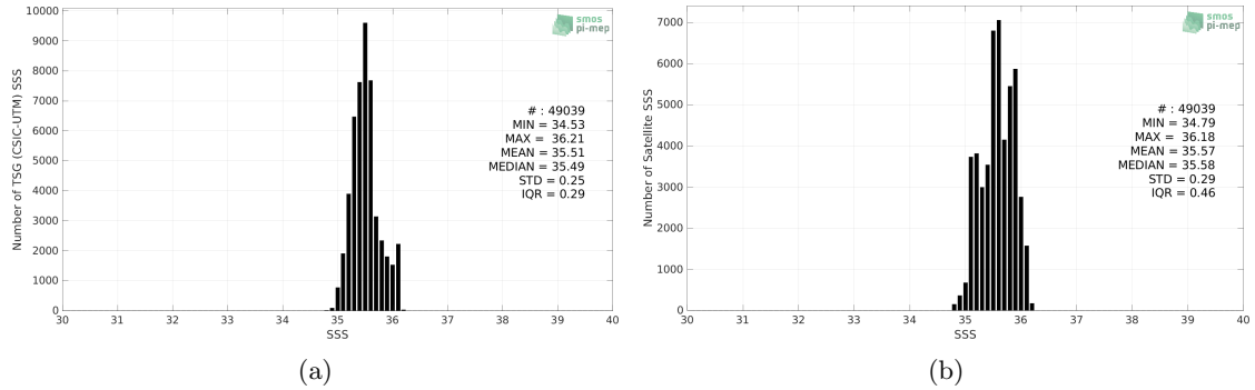
Figure 2: Histograms of SSS from TSG (CSIC-UTM) (a) and SMOS SSS L4 v2 - Daily (BEC) (b) considering all match-up pairs per bins of 0.1 over the Indian Ocean Pi-MEP region and for the full satellite product period.
