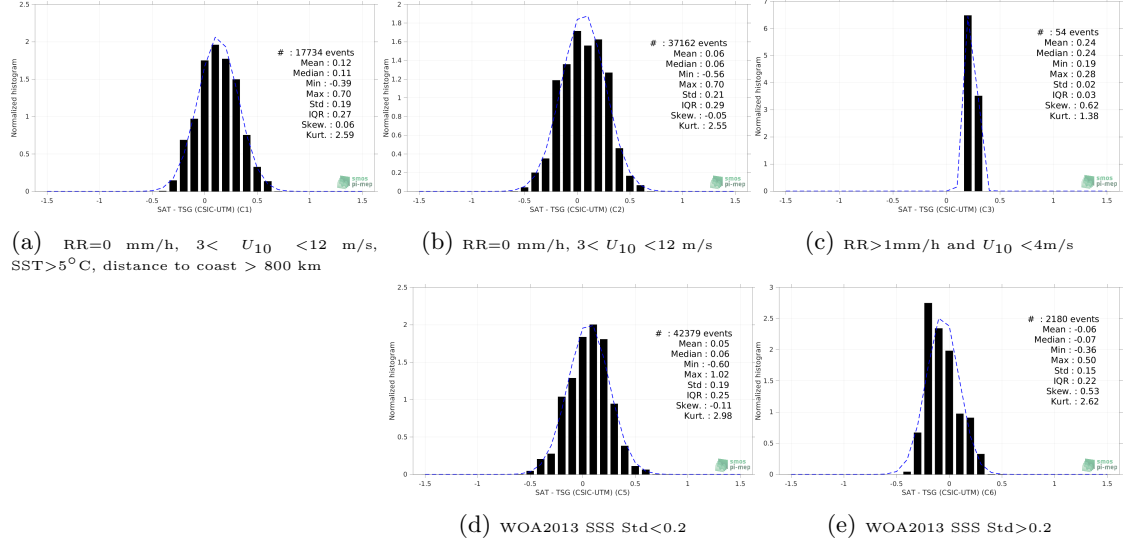
Figure 13: Normalized histogram of \Delta SSS (SMOS SSS L4 v2 - Daily (BEC) - TSG (CSIC-UTM)) for 5 different subdatasets corresponding to: RR=0 mm/h, 3 < U_{10} < 12 m/s, SST > 5°C, distance to coast > 800 km (a), RR=0 mm/h, 3 < U_{10} < 12 m/s (b), RR > 1mm/h and U_{10} < 4 m/s (c), WOA2013 SSS Std < 0.2 (d), WOA2013 SSS Std > 0.2 (e).
