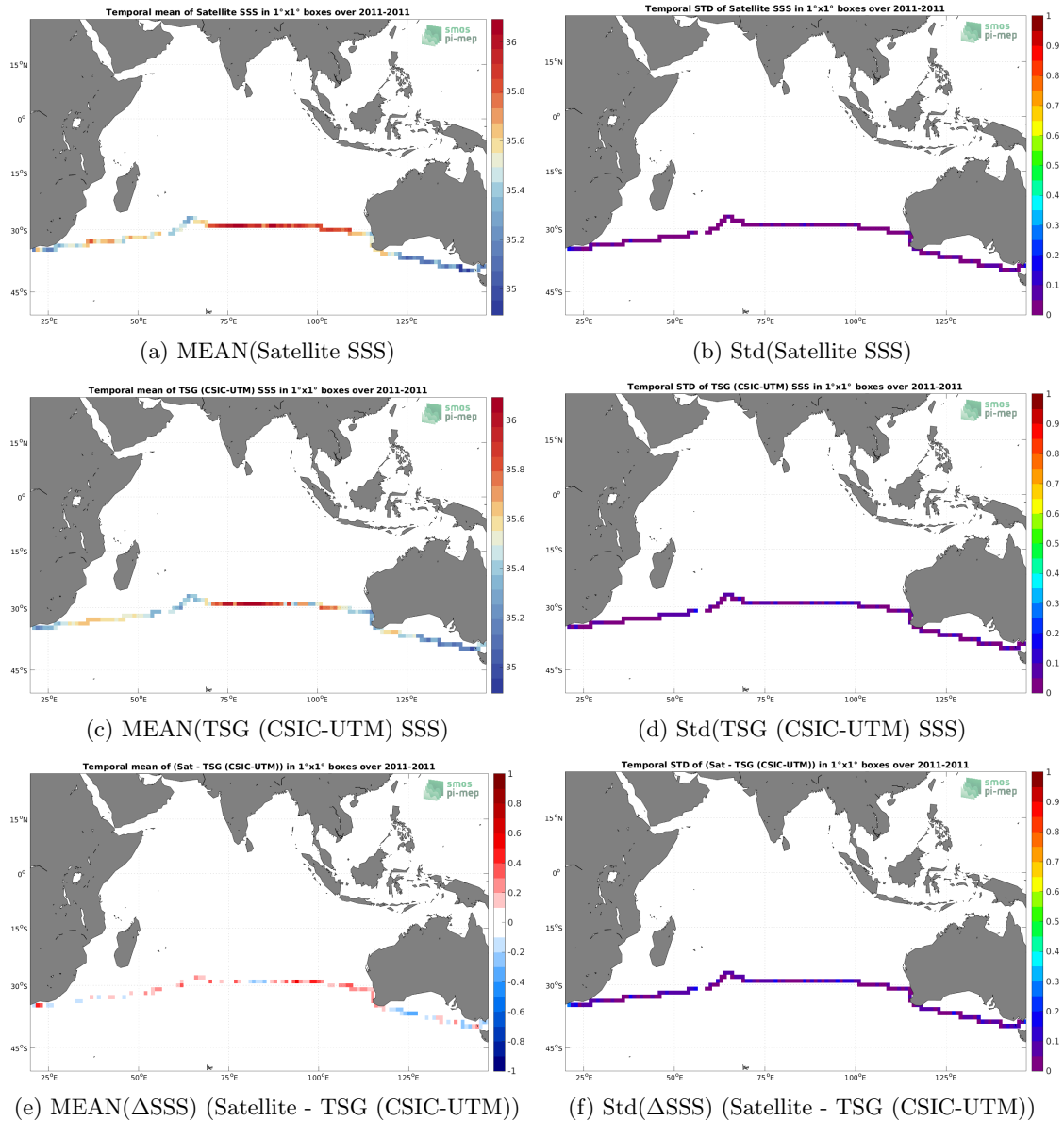
Figure 6: Temporal mean (left) and Std (right) of SSS from SMOS SSS L4 v2 - Daily (BEC) (top), TSG (CSIC-UTM) (middle), and of \Delta SSS (Satellite - TSG (CSIC-UTM)). Only match-up pairs are used to generate these maps.
