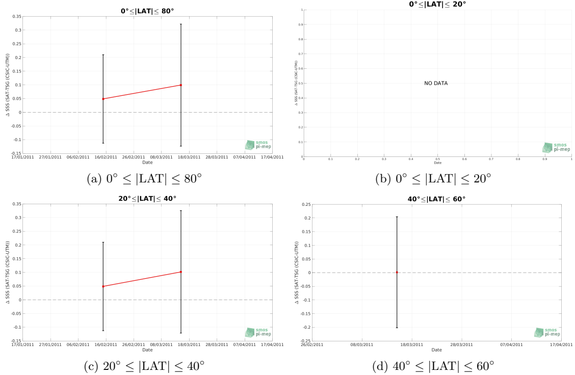
Figure 10: Monthly median (red curves) of \Delta\text{SSS} (Satellite - TSG (CSIC-UTM)) and \pm 1 Std (black vertical thick bars) as function of time for all the collected Pi-MEP match-up pairs estimated over the Indian Ocean Pi-MEP region and for the full satellite product period are shown for different latitude bands: (a) 80^{\circ}\text{S}-80^{\circ}\text{N} , (b) 20^{\circ}\text{S}-20^{\circ}\text{N} , (c) 40^{\circ}\text{S}-20^{\circ}\text{S} and 20^{\circ}\text{N}-40^{\circ}\text{N} and (d) 60^{\circ}\text{S}-40^{\circ}\text{S} and 40^{\circ}\text{N}-60^{\circ}\text{N} .
