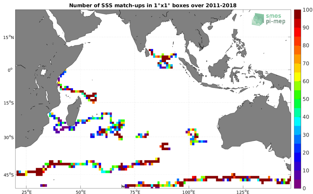
Figure 3: Number of SSS match-ups between Surface drifters SSS and the SMOS SSS L4 v2 - Daily (BEC) SSS product for the Indian Ocean Pi-MEP region over 1^\circ \times 1^\circ boxes and for the full satellite product period.
