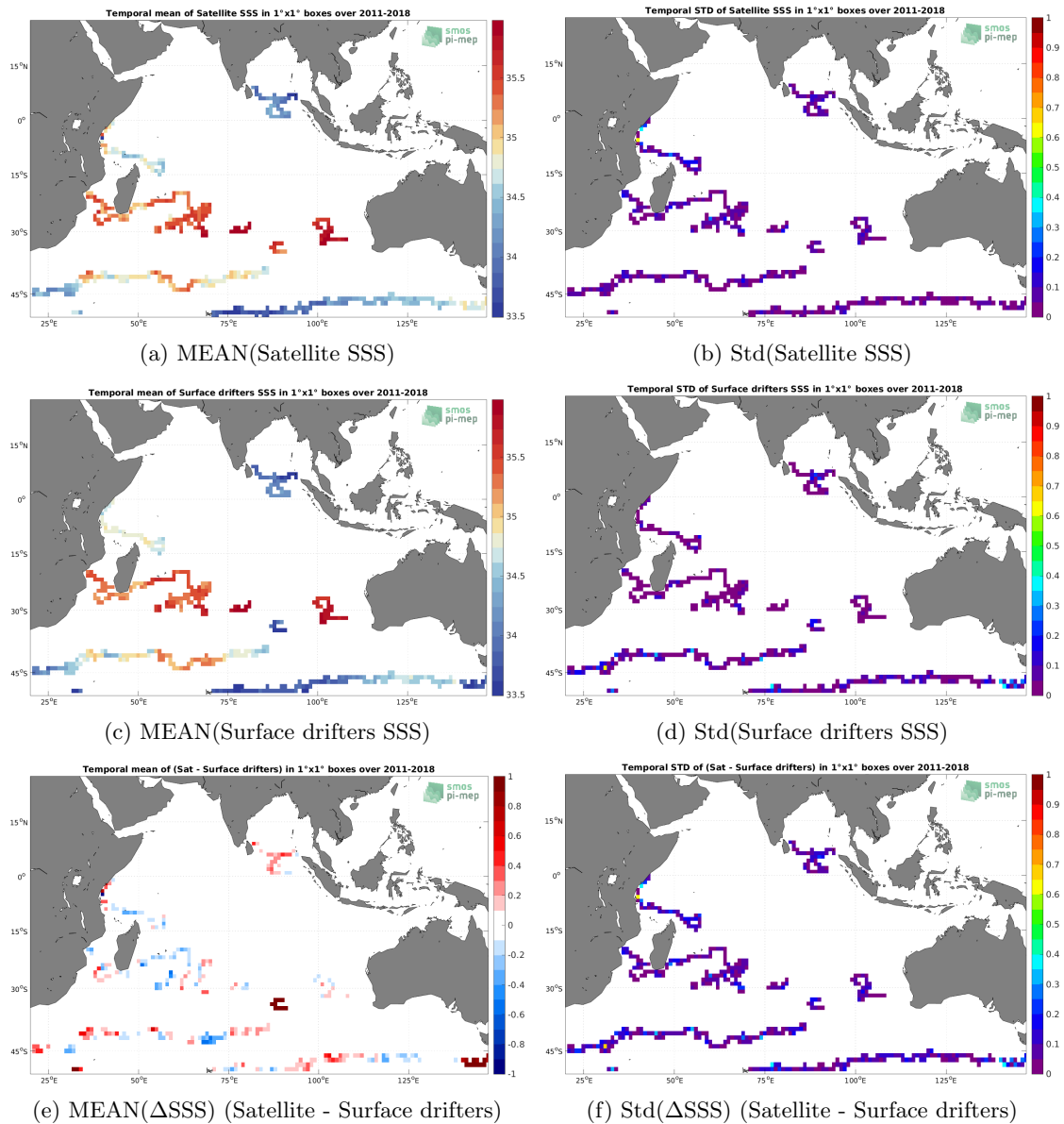
Figure 5: Temporal mean (left) and Std (right) of SSS from SMOS SSS L4 v2 - Daily (BEC) (top), Surface drifters (middle), and of \Delta SSS (Satellite - Surface drifters). Only match-up pairs are used to generate these maps.
