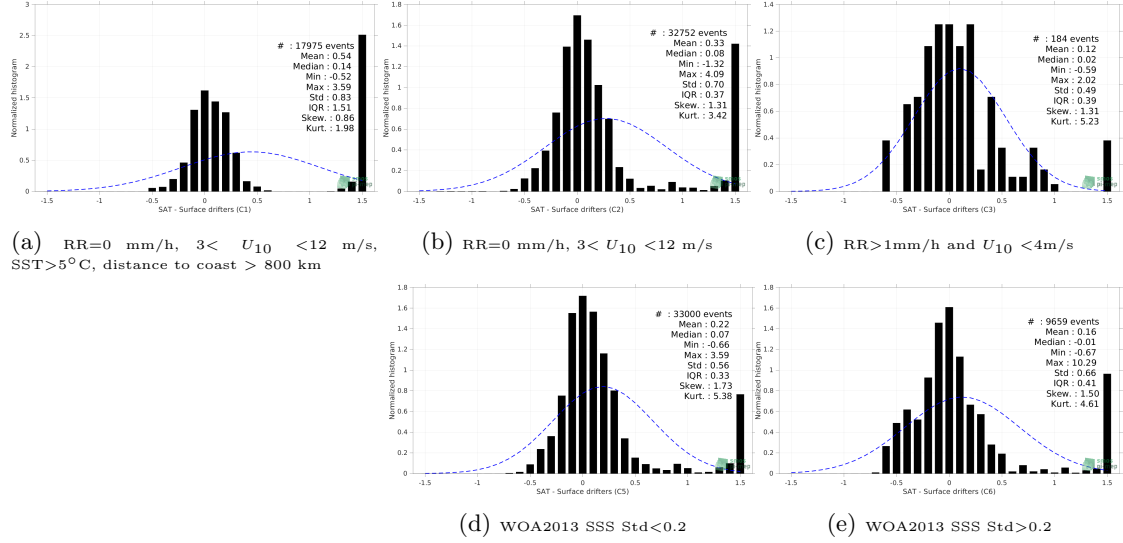
Figure 12: Normalized histogram of \Delta SSS (SMOS SSS L4 v2 - Daily (BEC) - Surface drifters) for 5 different subdatasets corresponding to: RR=0 mm/h, 3 < U_{10} < 12 m/s, SST > 5°C, distance to coast > 800 km (a), RR=0 mm/h, 3 < U_{10} < 12 m/s (b), RR > 1mm/h and U_{10} < 4 m/s (c), WOA2013 SSS Std < 0.2 (d), WOA2013 SSS Std > 0.2 (e).
