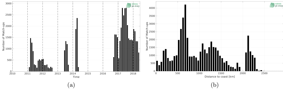
Figure 1: Number of match-ups between Surface drifters and SMOS SSS L4 v2 - Daily (BEC) SSS as a function of time (a) and as function of the distance to coast (b) over the Indian Ocean Pi-MEP region and for the full satellite product period.
