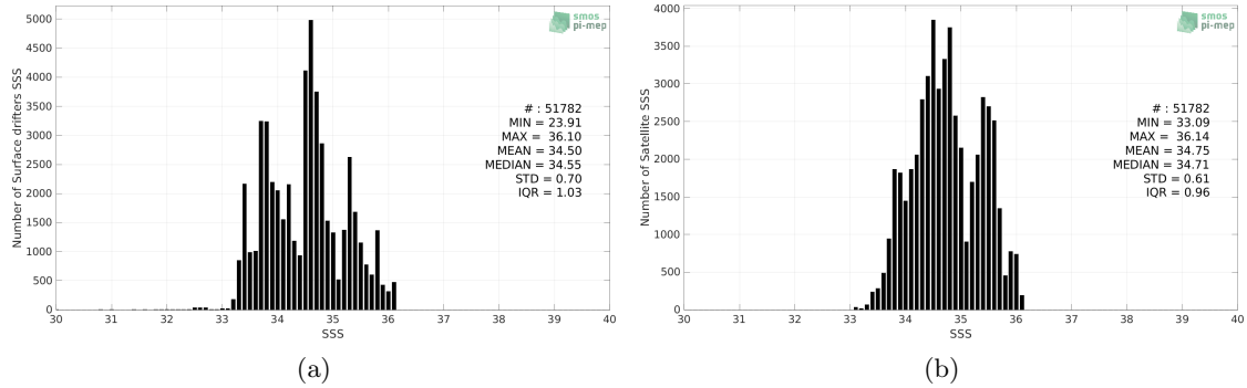
Figure 2: Histograms of SSS from Surface drifters (a) and SMOS SSS L4 v2 - Daily (BEC) (b) considering all match-up pairs per bins of 0.1 over the Indian Ocean Pi-MEP region and for the full satellite product period.
