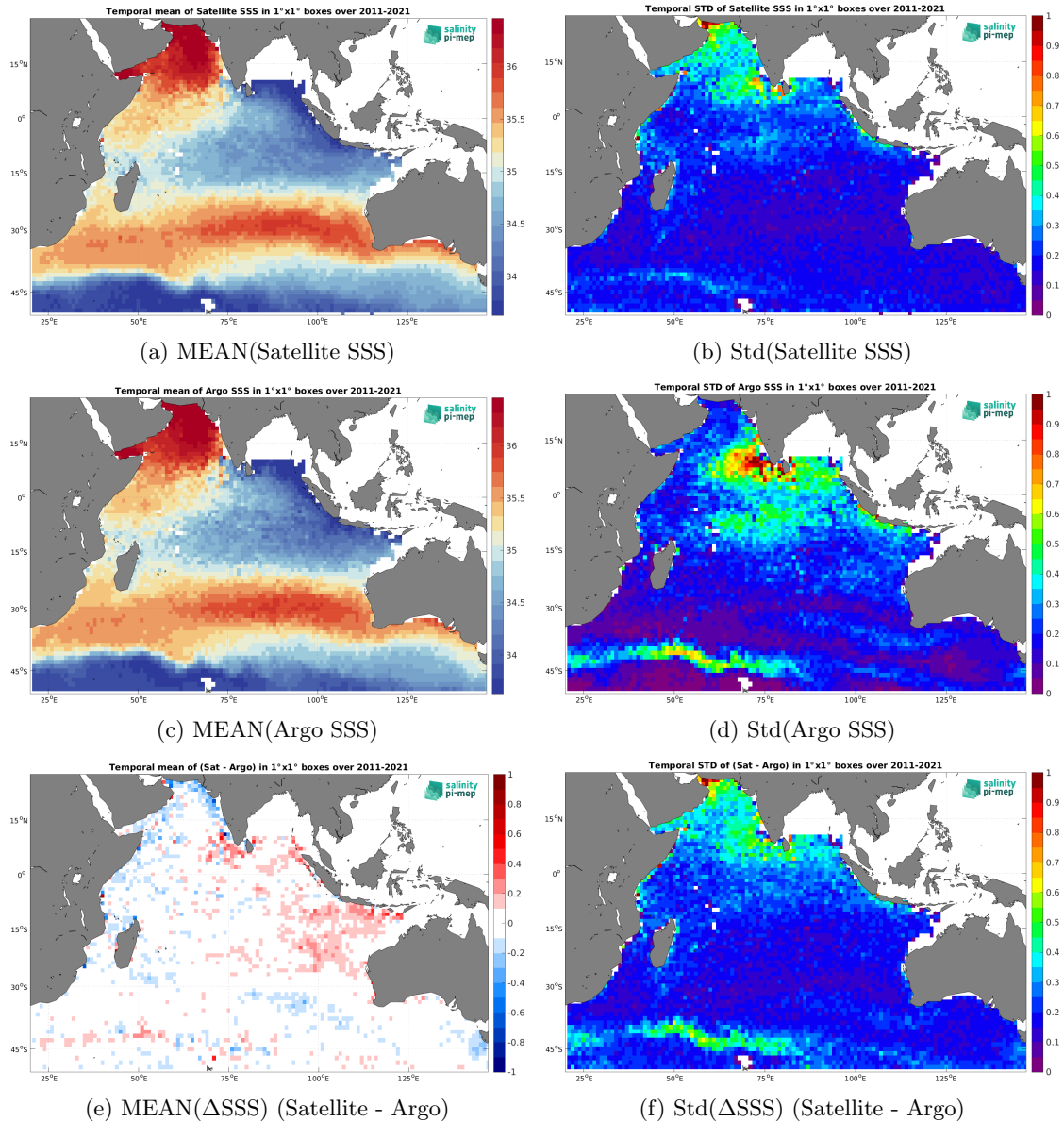
Figure 6: Temporal mean (left) and Std (right) of SSS from SMOS SSS L4 v2 - Daily (BEC) (top), Argo (middle), and of \Delta SSS (Satellite - Argo). Only match-up pairs are used to generate these maps.
