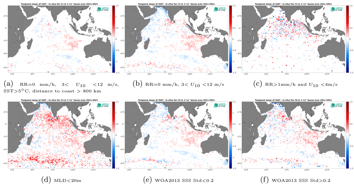
Figure 12: Temporal mean gridded over spatial boxes of size 1^\circ \times 1^\circ of \Delta SSS (SMOS SSS L4 v2 - Daily (BEC) - Argo) for 6 different subdatasets corresponding to:RR=0 mm/h, 3 < U_{10} < 12 m/s, SST >5^\circ C, distance to coast > 800 km (a), RR=0 mm/h, 3 < U_{10} < 12 m/s (b), RR >1 mm/h and U_{10} < 4 m/s (c),MLD <20 m (d),WOA2013 SSS Std <0.2 (e),WOA2013 SSS Std >0.2 (f).
