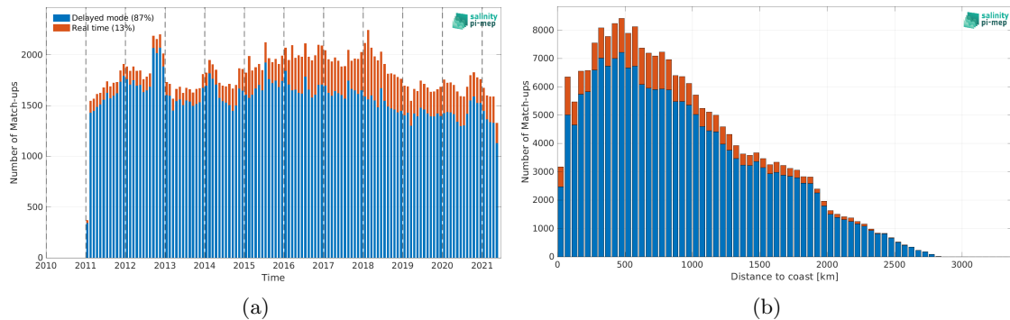
Figure 1: Number of match-ups between Argo and SMOS SSS L4 v2 - Daily (BEC) SSS as a function of time (a) and as function of the distance to coast (b) over the Indian Ocean Pi-MEP region and for the full satellite product period.
