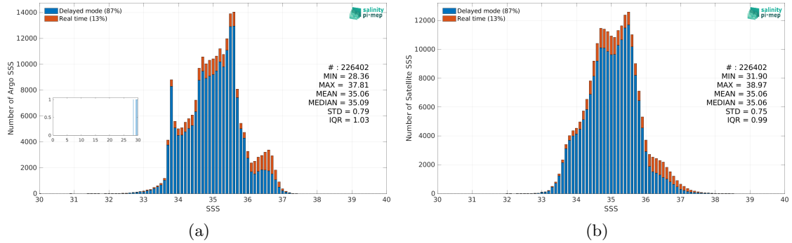
Figure 2: Histograms of SSS from Argo (a) and SMOS SSS L4 v2 - Daily (BEC) (b) considering all match-up pairs per bins of 0.1 over the Indian Ocean Pi-MEP region and for the full satellite product period.
