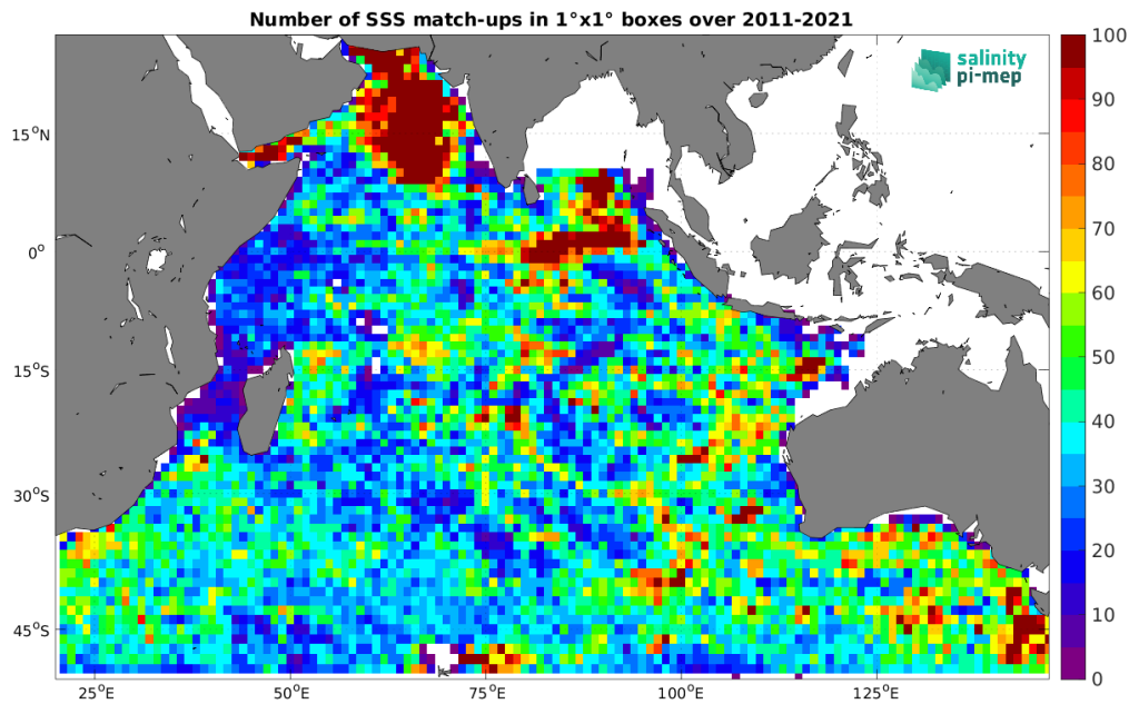
Figure 4: Number of SSS match-ups between Argo SSS and the SMOS SSS L4 v2 - Daily (BEC) SSS product for the Indian Ocean Pi-MEP region over 1^\circ \times 1^\circ boxes and for the full satellite product period.
