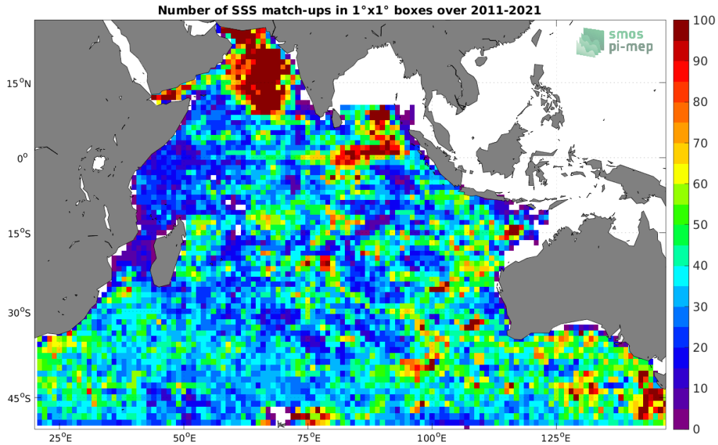
Figure 4: Number of SSS match-ups between Argo SSS and the SMOS SSS L4 v2 - Daily (BEC) SSS product for the Indian Ocean Pi-MEP region over 1^\circ \times 1^\circ boxes and for the full satellite product period.
