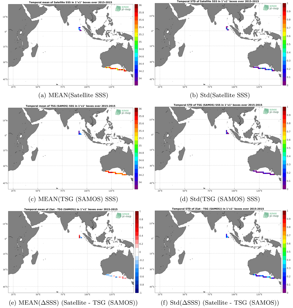
Figure 6: Temporal mean (left) and Std (right) of SSS from SMOS SSS L3 v3 Monthly (ICDC) (top), TSG (SAMOS) (middle), and of \Delta SSS (Satellite - TSG (SAMOS)). Only match-up pairs are used to generate these maps.
