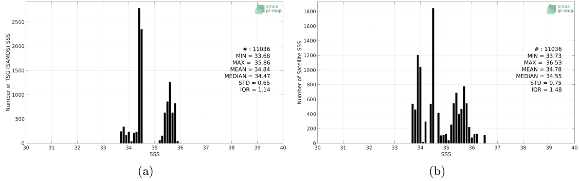
Figure 2: Histograms of SSS from TSG (SAMOS) (a) and SMOS SSS L3 v3 Monthly (ICDC) (b) considering all match-up pairs per bins of 0.1 over the Indian Ocean Pi-MEP region and for the full satellite product period.
