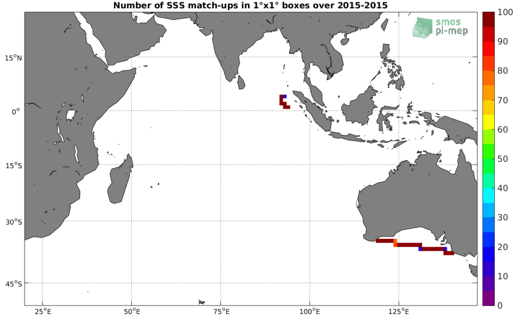
Figure 4: Number of SSS match-ups between TSG (SAMOS) SSS and the SMOS SSS L3 v3 Monthly (ICDC) SSS product for the Indian Ocean Pi-MEP region over 1^\circ \times 1^\circ boxes and for the full satellite product period.
