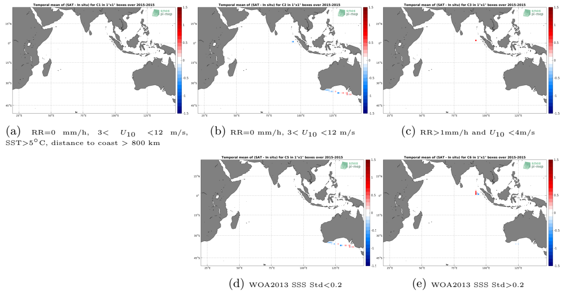
Figure 12: Temporal mean gridded over spatial boxes of size 1^\circ \times 1^\circ of \Delta SSS (SMOS SSS L3 v3 Monthly (ICDC) - TSG (SAMOS)) for 5 different subdatasets corresponding to: RR=0 mm/h, 3 < U_{10} < 12 m/s, SST > 5^\circ C , distance to coast > 800 km (a), RR=0 mm/h, 3 < U_{10} < 12 m/s (b), RR > 1 mm/h and U_{10} < 4 m/s (c), WOA2013 SSS Std < 0.2 (d), WOA2013 SSS Std > 0.2 (e).
