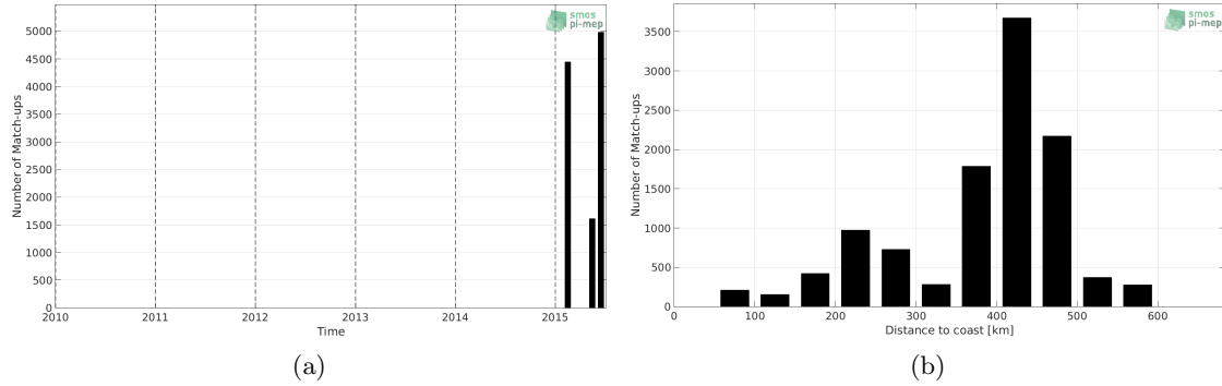
Figure 1: Number of match-ups between TSG (SAMOS) and SMOS SSS L3 v3 Monthly (ICDC) SSS as a function of time (a) and as function of the distance to coast (b) over the Indian Ocean Pi-MEP region and for the full satellite product period.
