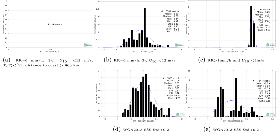
Figure 13: Normalized histogram of \Delta\text{SSS} (SMOS SSS L3 v3 Monthly (ICDC) - TSG (SAMOS)) for 5 different subdatasets corresponding to: RR=0 mm/h, 3 < U_{10} < 12 m/s, SST > 5^\circ\text{C} , distance to coast > 800 km (a), RR=0 mm/h, 3 < U_{10} < 12 m/s (b), RR > 1\text{mm/h} and U_{10} < 4\text{m/s} (c), WOA2013 SSS Std < 0.2 (d), WOA2013 SSS Std > 0.2 (e).
