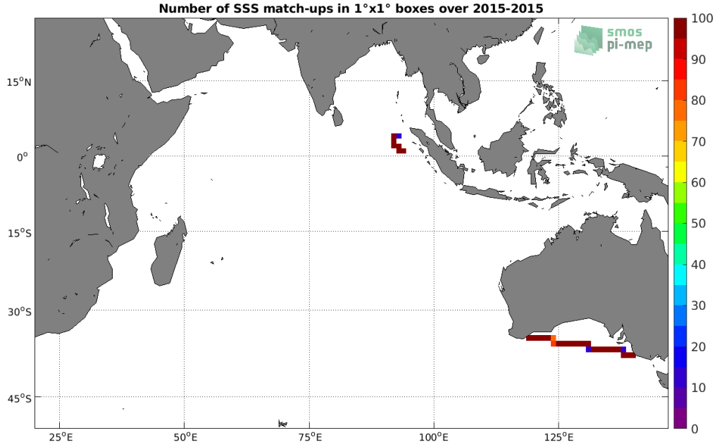
Figure 4: Number of SSS match-ups between TSG (SAMOS) SSS and the SMOS SSS L3 v3 Monthly (ICDC) SSS product for the Indian Ocean Pi-MEP region over 1^\circ \times 1^\circ boxes and for the full satellite product period.
