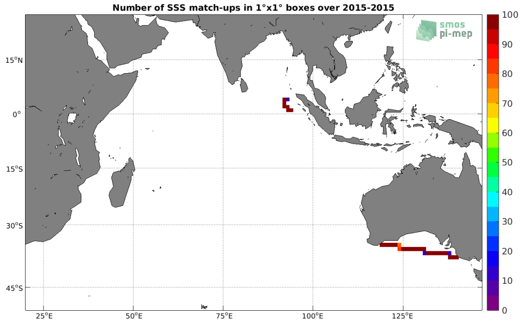
Figure 4: Number of SSS match-ups between TSG (SAMOS) SSS and the SMOS SSS L3 v3 Monthly (ICDC) SSS product for the Indian Ocean Pi-MEP region over 1°x1° boxes and for the full satellite product period.
