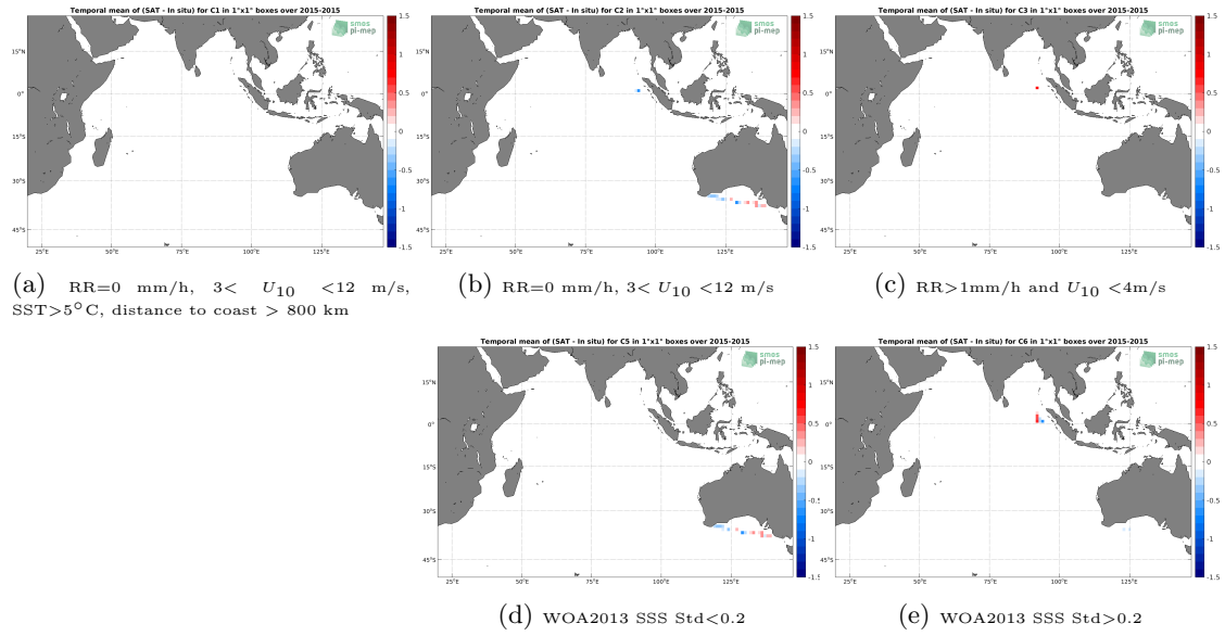
Figure 12: Temporal mean gridded over spatial boxes of size 1^\circ \times 1^\circ of \Delta SSS (SMOS SSS L3 v3 Monthly (ICDC) - TSG (SAMOS)) for 5 different subdatasets corresponding to:RR=0 mm/h, 3 < U_{10} < 12 m/s, SST>5°C, distance to coast > 800 km (a), RR=0 mm/h, 3 < U_{10} < 12 m/s (b), RR>1mm/h and U_{10} < 4 m/s (c), WOA2013 SSS Std<0.2 (d), WOA2013 SSS Std>0.2 (e).
