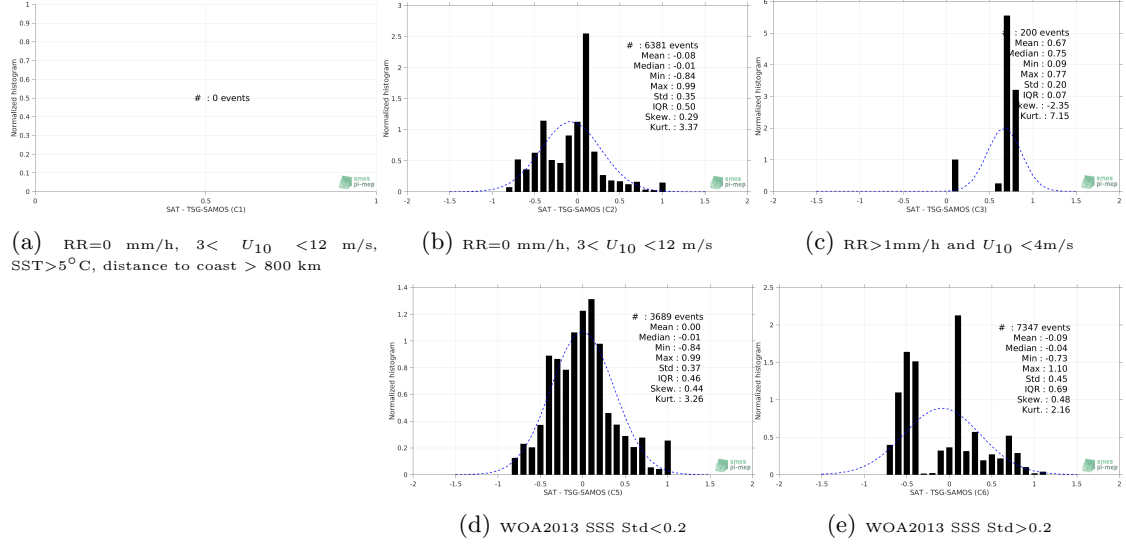
Figure 13: Normalized histogram of \Delta\text{SSS} (SMOS-L3-ICDC-V3-MONTHLY-0.5DEG - TSG-SAMOS) for 5 different subdatasets corresponding to: RR=0 mm/h, 3 < U_{10} < 12 m/s, SST > 5^{\circ}\text{C} , distance to coast > 800 km (a), RR=0 mm/h, 3 < U_{10} < 12 m/s (b), RR > 1\text{mm/h} and U_{10} < 4\text{m/s} (c), WOA2013 SSS Std <0.2 (d), WOA2013 SSS Std >0.2 (e).
