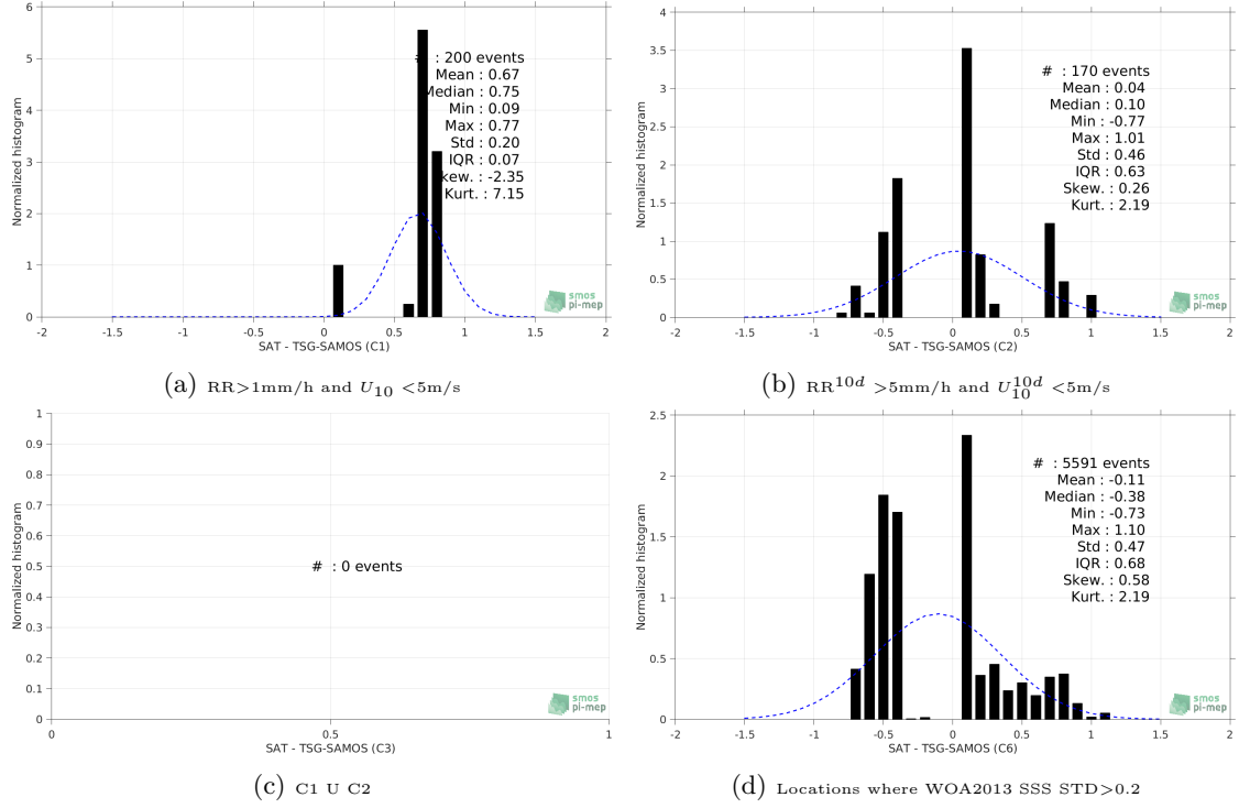
Figure 13: Normalized histogram of \Delta\text{SSS} (SMOS-L3-ICDC-V3-MONTHLY-0.5DEG - TSG-SAMOS) for 6 different subdatasets corresponding to: RR > 1\text{mm/h} and U_{10} < 5\text{m/s} (a), RR^{10d} > 5\text{mm/h} and U_{10}^{10d} < 5\text{m/s} (b), C1 U C2 (c), Locations where WOA2013 SSS STD > 0.2 (d).
