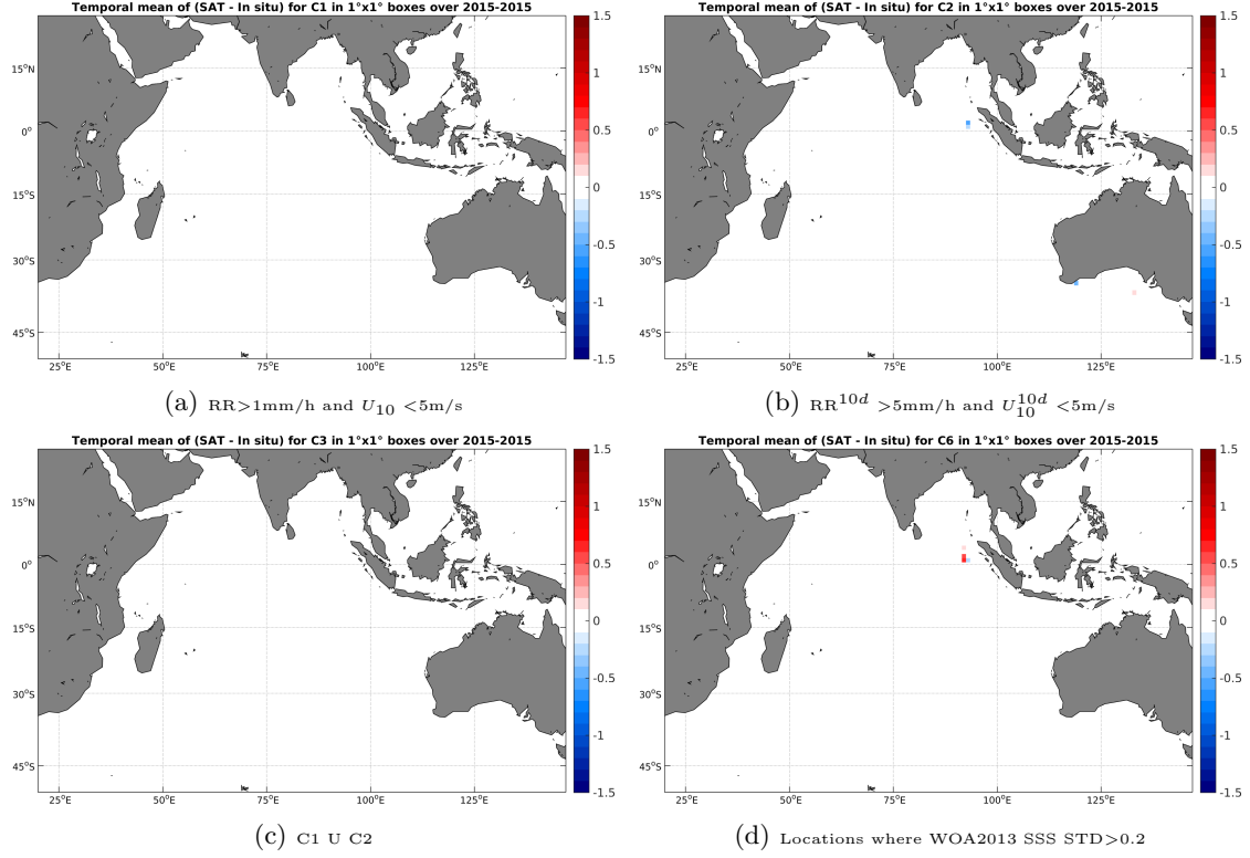
Figure 12: Temporal mean gridded over spatial boxes of size 1^\circ \times 1^\circ of \Delta SSS (SMOS-L3-ICDC-V3-MONTHLY-0.5DEG - TSG-SAMOS) for 4 different subdatasets corresponding to: RR > 1\text{mm/h} and U_{10} < 5\text{m/s} (a), RR^{10d} > 5\text{mm/h} and U_{10}^{10d} < 5\text{m/s} (b), C1 U C2 (c), Locations where WOA2013 SSS STD > 0.2 (d).
