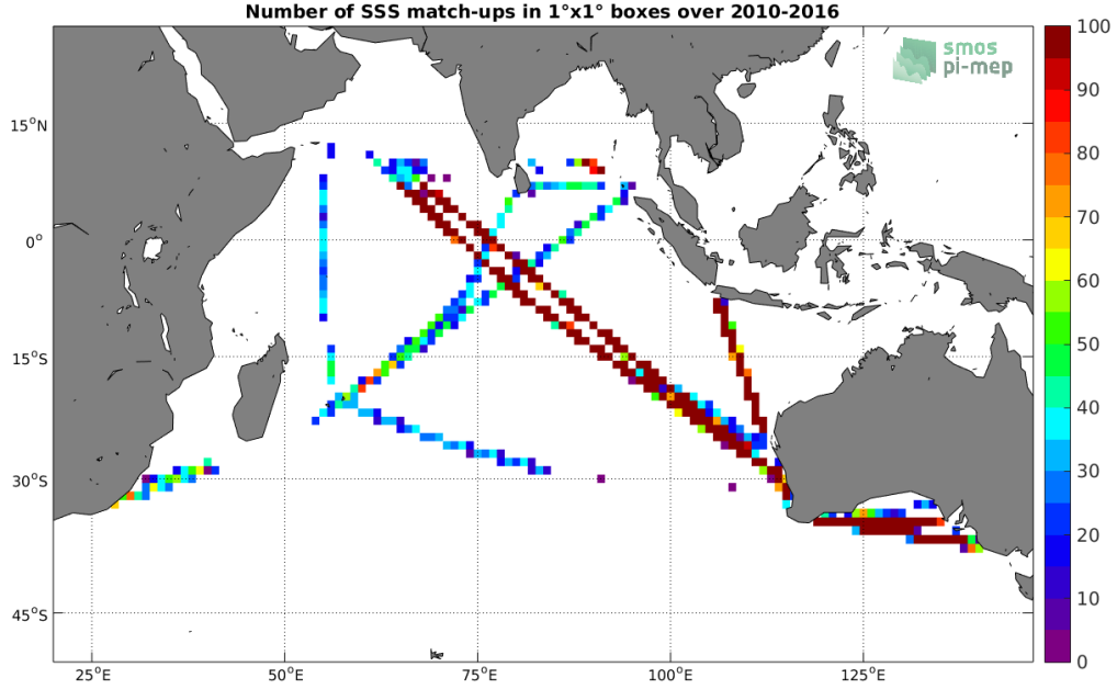
Figure 4: Number of SSS match-ups between TSG (LEGOS-DM) SSS and the SMOS SSS L3 v3 Monthly (ICDC) SSS product for the Indian Ocean Pi-MEP region over 1^\circ \times 1^\circ boxes and for the full satellite product period.
