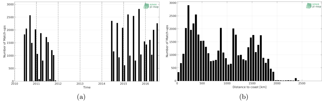
Figure 1: Number of match-ups between TSG (LEGOS-DM) and SMOS SSS L3 v3 Monthly (ICDC) SSS as a function of time (a) and as function of the distance to coast (b) over the Indian Ocean Pi-MEP region and for the full satellite product period.
