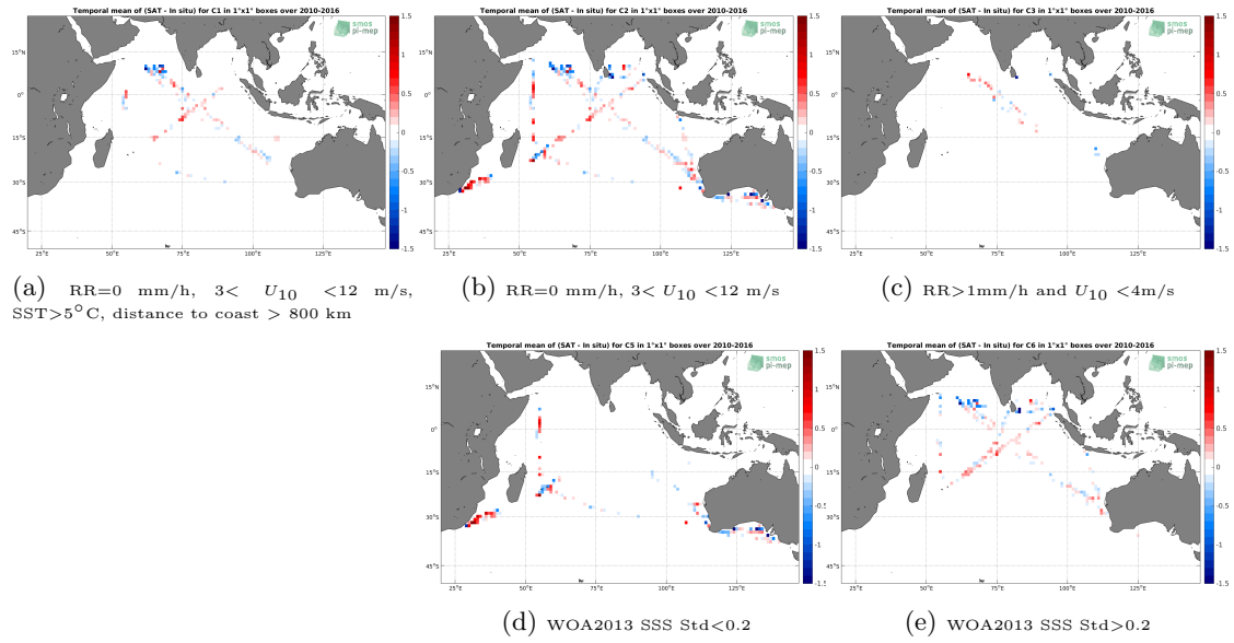
Figure 12: Temporal mean gridded over spatial boxes of size 1^\circ \times 1^\circ of \Delta SSS (SMOS SSS L3 v3 Monthly (ICDC) - TSG (LEGOS-DM)) for 5 different subdatasets corresponding to: RR=0 mm/h, 3 < U_{10} < 12 m/s, SST > 5^\circ C , distance to coast > 800 km (a), RR=0 mm/h, 3 < U_{10} < 12 m/s (b), RR > 1 mm/h and U_{10} < 4 m/s (c), WOA2013 SSS Std < 0.2 (d), WOA2013 SSS Std > 0.2 (e).
