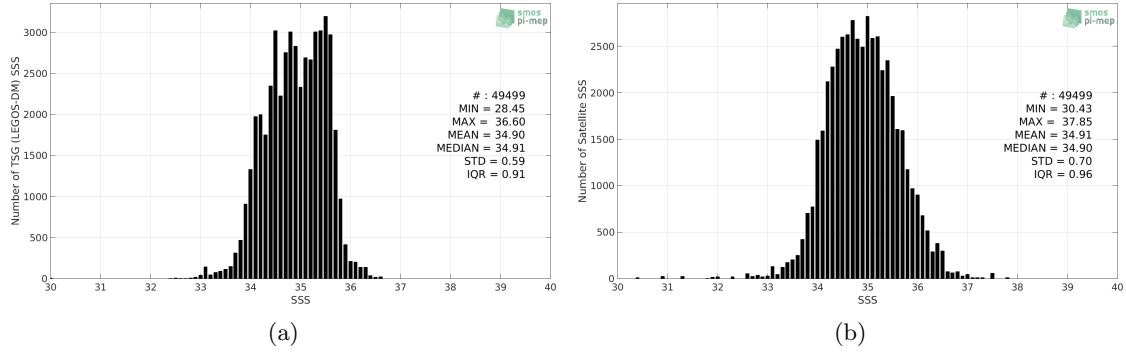
Figure 2: Histograms of SSS from TSG (LEGOS-DM) (a) and SMOS SSS L3 v3 Monthly (ICDC) (b) considering all match-up pairs per bins of 0.1 over the Indian Ocean Pi-MEP region and for the full satellite product period.
