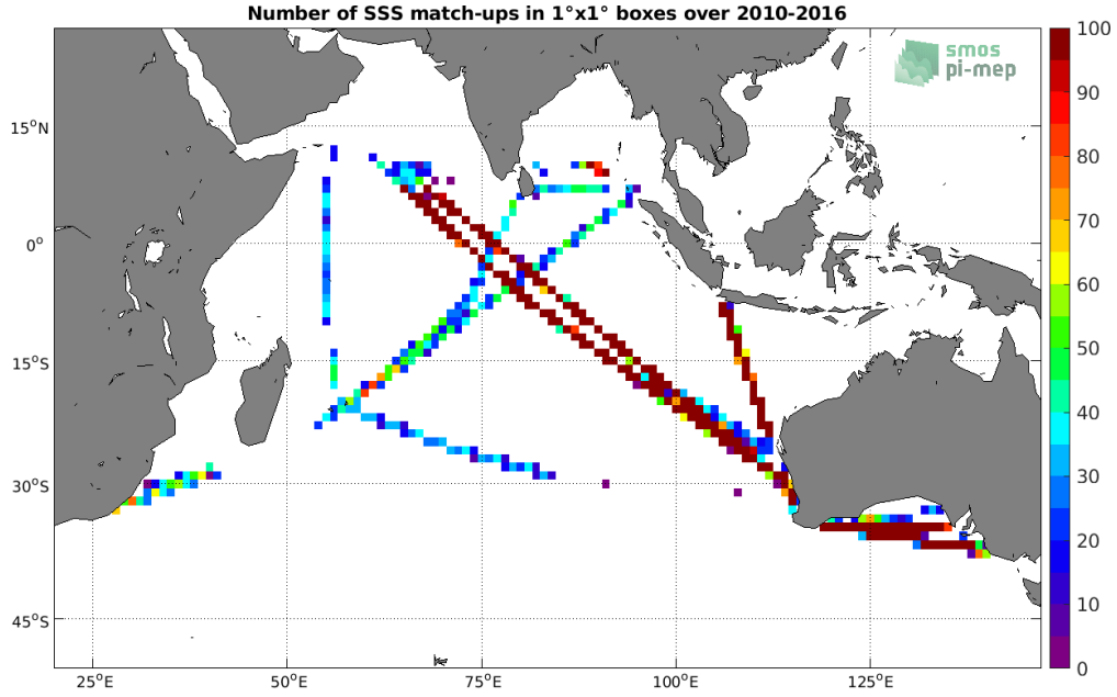
Figure 4: Number of SSS match-ups between TSG (LEGOS-DM) SSS and the SMOS SSS L3 v3 Monthly (ICDC) SSS product for the Indian Ocean Pi-MEP region over 1^\circ \times 1^\circ boxes and for the full satellite product period.
