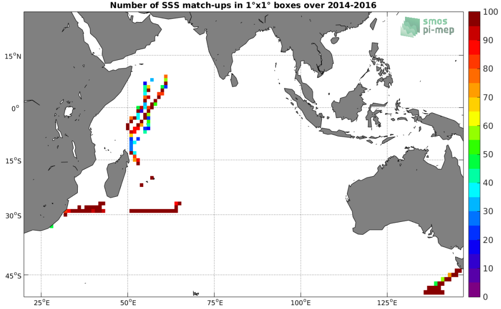
Figure 4: Number of SSS match-ups between TSG (GOSUD-Research-vessel) SSS and the SMOS SSS L3 v3 Monthly (ICDC) SSS product for the Indian Ocean Pi-MEP region over 1^\circ \times 1^\circ boxes and for the full satellite product period.
