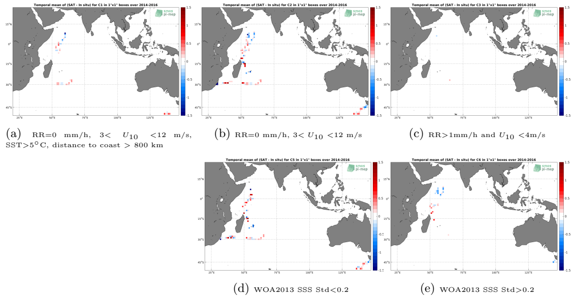
Figure 12: Temporal mean gridded over spatial boxes of size 1^\circ \times 1^\circ of \Delta SSS (SMOS-L3-ICDC-V3-MONTHLY-0.5DEG - TSG-GOSUD-Research-vessel) for 5 different subdatasets corresponding to:RR=0 mm/h, 3 < U_{10} < 12 m/s, SST >5^\circ C, distance to coast > 800 km (a), RR=0 mm/h, 3 < U_{10} < 12 m/s (b), RR >1 mm/h and U_{10} < 4 m/s (c), WOA2013 SSS Std <0.2 (d), WOA2013 SSS Std >0.2 (e).
