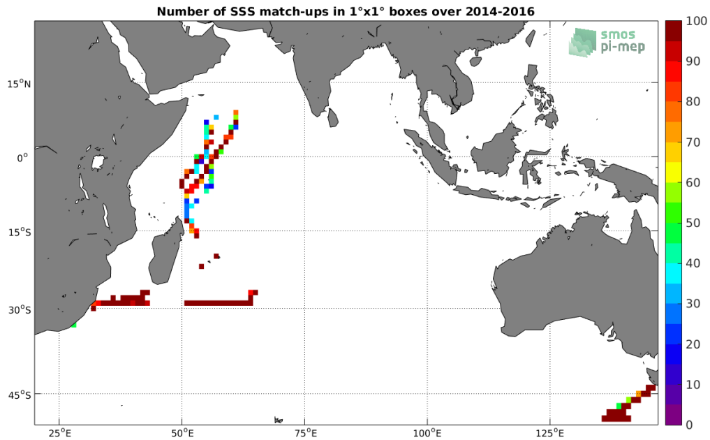
Figure 4: Number of SSS match-ups between TSG-GOSUD-Research-vessel SSS and the SMOS-L3-ICDC-V3-MONTHLY-0.5DEG SSS product for the Indian Ocean Pi-MEP region over 1^\circ \times 1^\circ boxes and for the full satellite product period.
