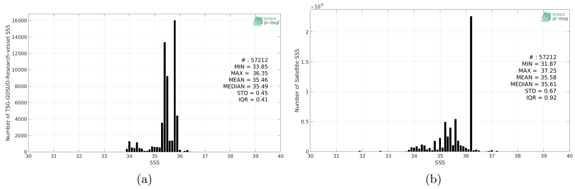
Figure 2: Histograms of SSS from TSG-GOSUD-Research-vessel (a) and SMOS-L3-ICDC-V3-MONTHLY-0.5DEG (b) considering all match-up pairs per bins of 0.1 over the Indian Ocean Pi-MEP region and for the full satellite product period.
