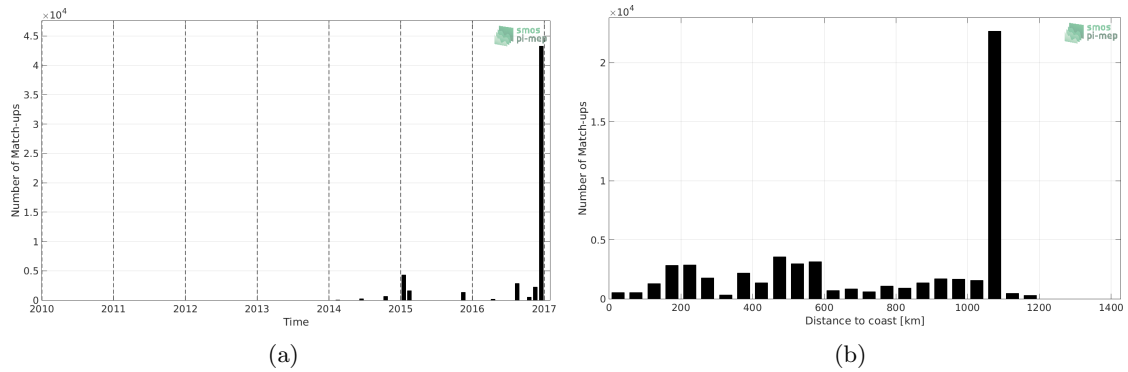
Figure 1: Number of match-ups between TSG-GOSUD-Research-vessel and SMOS-L3-ICDC-V3-MONTHLY-0.5DEG SSS as a function of time (a) and as function of the distance to coast (b) over the Indian Ocean Pi-MEP region and for the full satellite product period.
