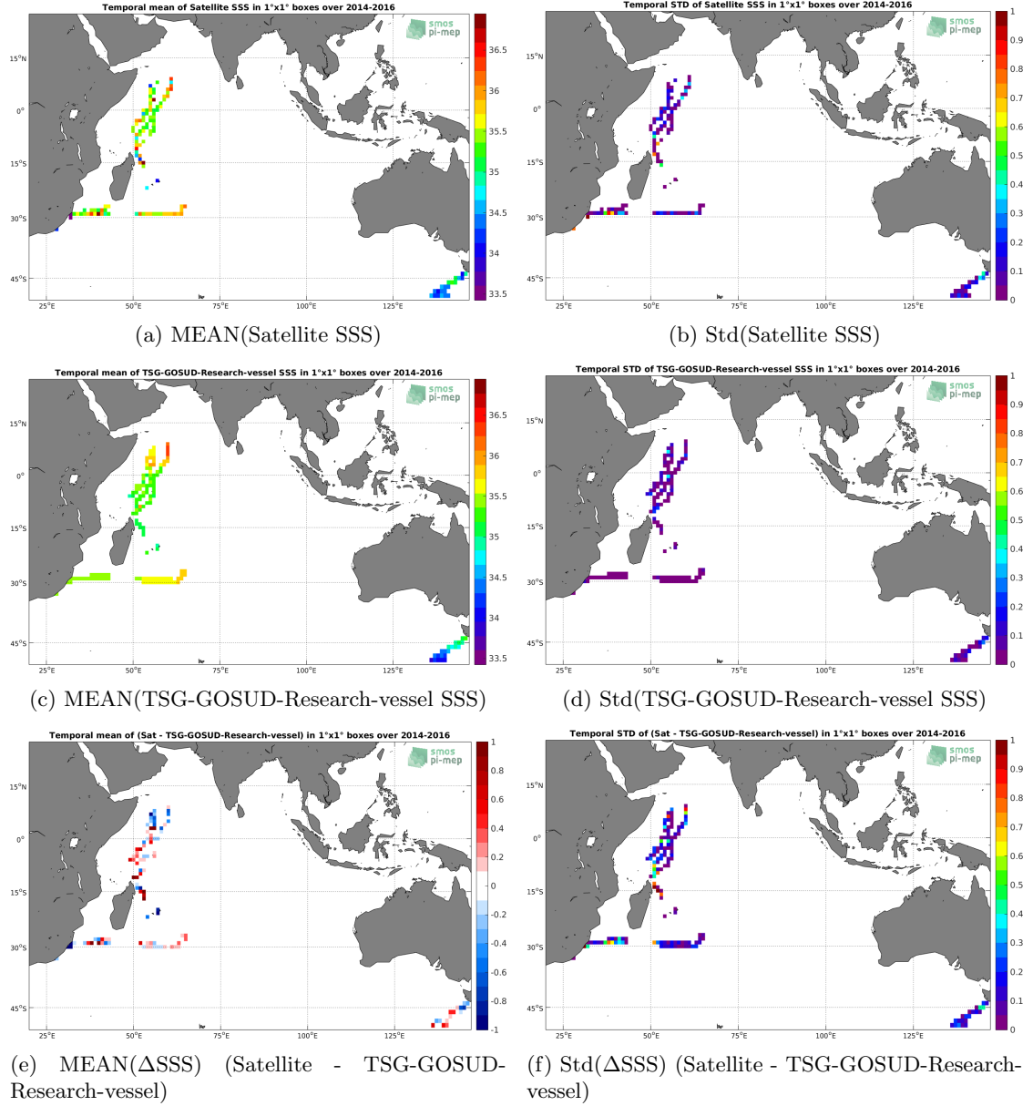
Figure 6: Temporal mean (left) and Std (right) of SSS from SMOS-L3-ICDC-V3-MONTHLY-0.5DEG (top), TSG-GOSUD-Research-vessel (middle), and of \Delta SSS (Satellite - TSG-GOSUD-Research-vessel). Only match-up pairs are used to generate these maps.
