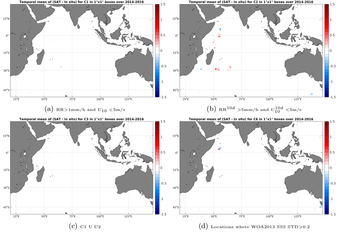
Figure 12: Temporal mean gridded over spatial boxes of size 1^\circ \times 1^\circ of \Delta SSS (SMOS-L3-ICDC-V3-MONTHLY-0.5DEG - TSG-GOSUD-Research-vessel) for 4 different subdatasets corresponding to: RR > 1 mm/h and U_{10} < 5 m/s (a), RR^{10d} > 5 mm/h and U_{10}^{10d} < 5 m/s (b), C1 U C2 (c), Locations where WOA2013 SSS STD > 0.2 (d).
