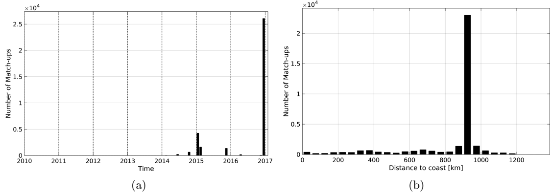
Figure 1: Number of match-ups between TSG-GOSUD-Research-vessel and SMOS-L3-ICDC-V3-MONTHLY-0.5DEG SSS as a function of time (a) and as function of the distance to coast (b) over the Indian Ocean Pi-MEP region and for the full satellite product period.
