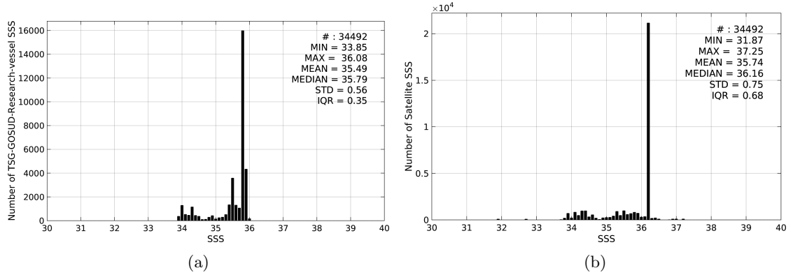
Figure 2: Histograms of SSS from TSG-GOSUD-Research-vessel (a) and SMOS-L3-ICDC-V3-MONTHLY-0.5DEG (b) considering all match-up pairs per bins of 0.1 over the Indian Ocean Pi-MEP region and for the full satellite product period.
