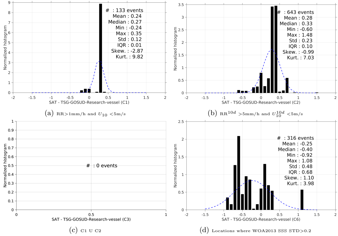
Figure 13: Normalized histogram of \Delta SSS (SMOS-L3-ICDC-V3-MONTHLY-0.5DEG - TSG-GOSUD-Research-vessel) for 6 different subdatasets corresponding to: RR>1mm/h and U_{10} < 5\text{m/s} (a), RR^{10d} > 5\text{mm/h} and U_{10}^{10d} < 5\text{m/s} (b), C1 U C2 (c), Locations where WOA2013 SSS STD>0.2 (d).
