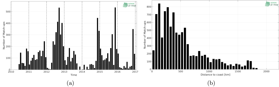
Figure 1: Number of match-ups between Marine mammals and SMOS SSS L3 v3 Monthly (ICDC) SSS as a function of time (a) and as function of the distance to coast (b) over the Indian Ocean Pi-MEP region and for the full satellite product period.
