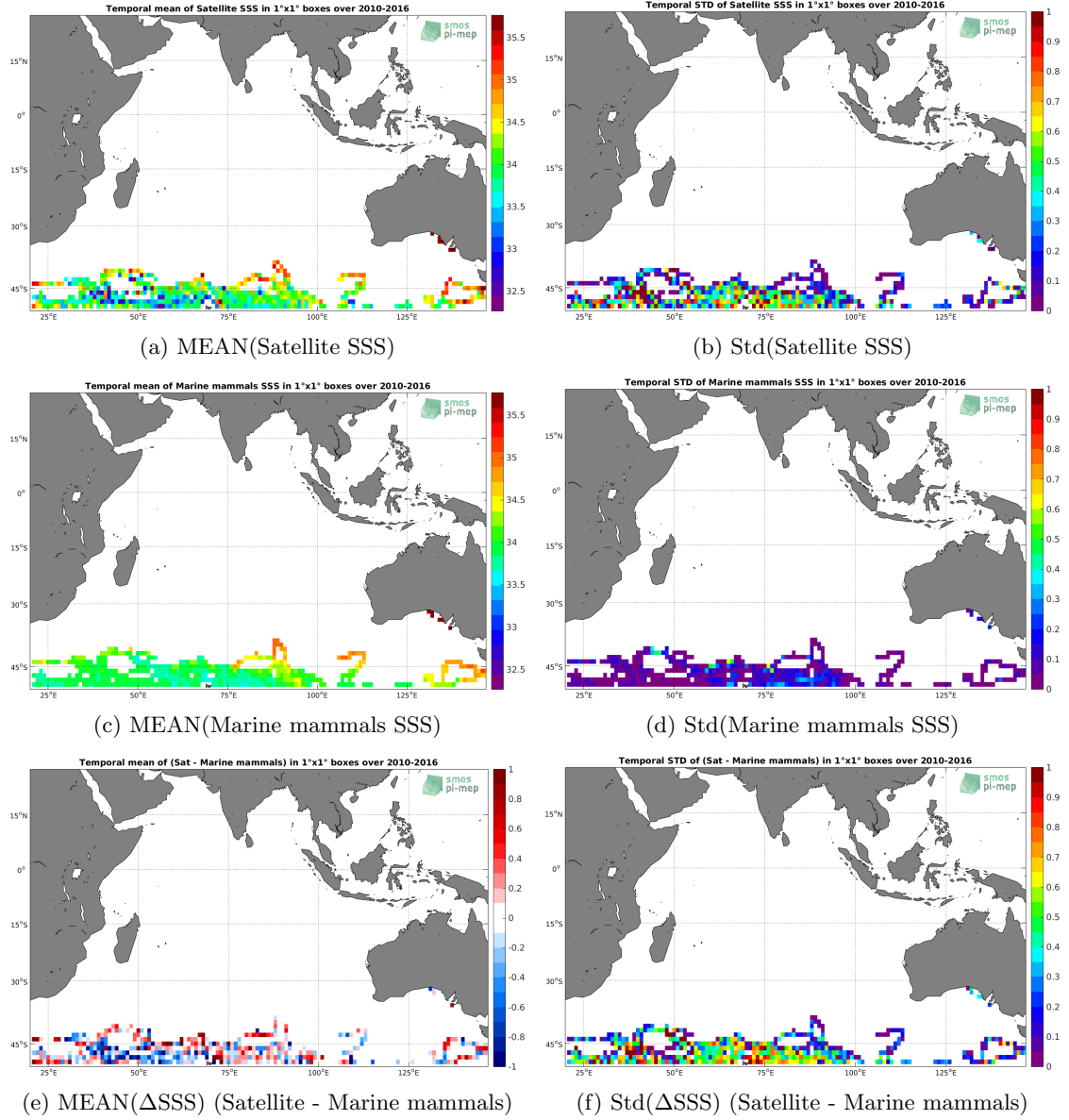
Figure 6: Temporal mean (left) and Std (right) of SSS from SMOS SSS L3 v3 Monthly (ICDC) (top), Marine mammals (middle), and of \Delta SSS (Satellite - Marine mammals). Only match-up pairs are used to generate these maps.
