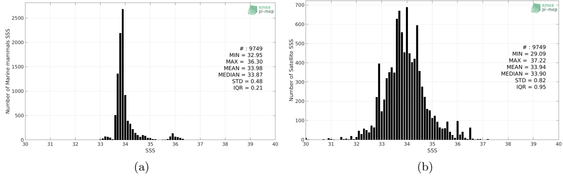
Figure 2: Histograms of SSS from Marine mammals (a) and SMOS SSS L3 v3 Monthly (ICDC) (b) considering all match-up pairs per bins of 0.1 over the Indian Ocean Pi-MEP region and for the full satellite product period.
