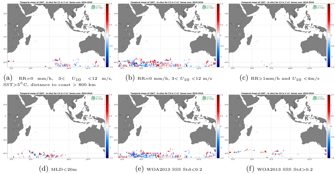
Figure 12: Temporal mean gridded over spatial boxes of size 1^\circ \times 1^\circ of \Delta SSS (SMOS SSS L3 v3 Monthly (ICDC) - Marine mammals) for 6 different subdatasets corresponding to: RR=0 mm/h, 3 < U_{10} < 12 m/s, SST > 5^\circ C , distance to coast > 800 km (a), RR=0 mm/h, 3 < U_{10} < 12 m/s (b), RR > 1 mm/h and U_{10} < 4 m/s (c), MLD < 20 m (d), WOA2013 SSS Std < 0.2 (e), WOA2013 SSS Std > 0.2 (f).
