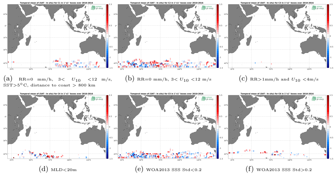
Figure 12: Temporal mean gridded over spatial boxes of size 1^{\circ}\times 1^{\circ} of \Delta\text{SSS} (SMOS SSS L3 v3 Monthly (ICDC) - Sea mammals) for 6 different subdatasets corresponding to: \text{RR}=0 mm/h, 3 < U_{10} < 12 m/s, \text{SST} > 5^{\circ}\text{C} , distance to coast > 800 km (a), \text{RR}=0 mm/h, 3 < U_{10} < 12 m/s (b), \text{RR} > 1\text{mm/h} and U_{10} < 4\text{m/s} (c), \text{MLD} < 20\text{m} (d), \text{WOA2013 SSS Std} < 0.2 (e), \text{WOA2013 SSS Std} > 0.2 (f).
