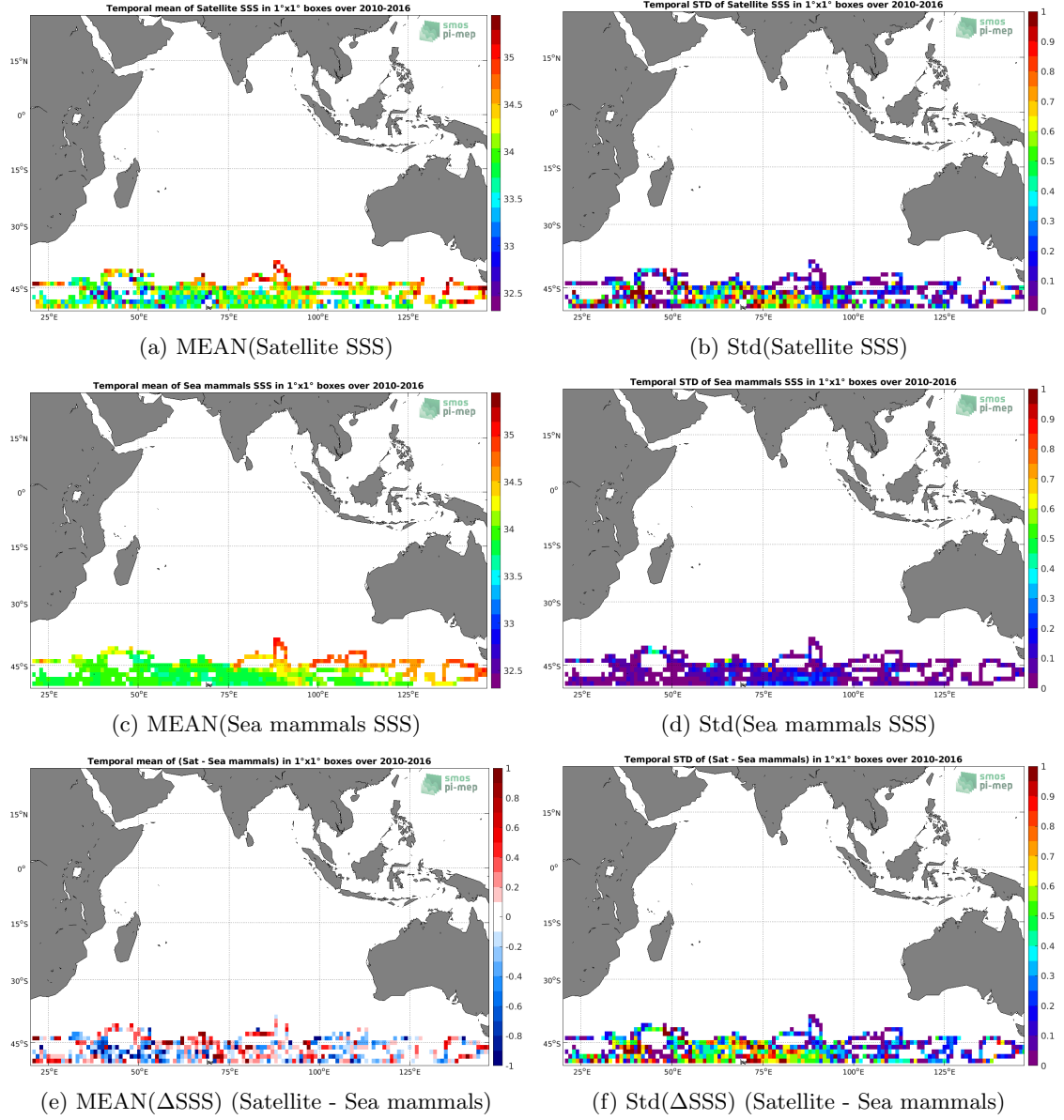
Figure 6: Temporal mean (left) and Std (right) of SSS from SMOS SSS L3 v3 Monthly (ICDC) (top), Sea mammals (middle), and of \Delta SSS (Satellite - Sea mammals). Only match-up pairs are used to generate these maps.
