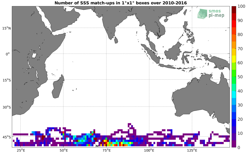
Figure 4: Number of SSS match-ups between Sea mammals SSS and the SMOS SSS L3 v3 Monthly (ICDC) SSS product for the Indian Ocean Pi-MEP region over 1^\circ \times 1^\circ boxes and for the full satellite product period.
