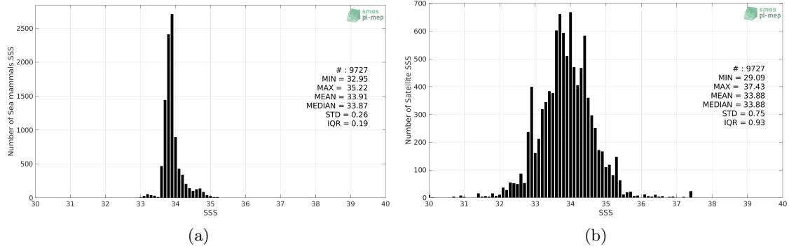
Figure 2: Histograms of SSS from Sea mammals (a) and SMOS SSS L3 v3 Monthly (ICDC) (b) considering all match-up pairs per bins of 0.1 over the Indian Ocean Pi-MEP region and for the full satellite product period.
