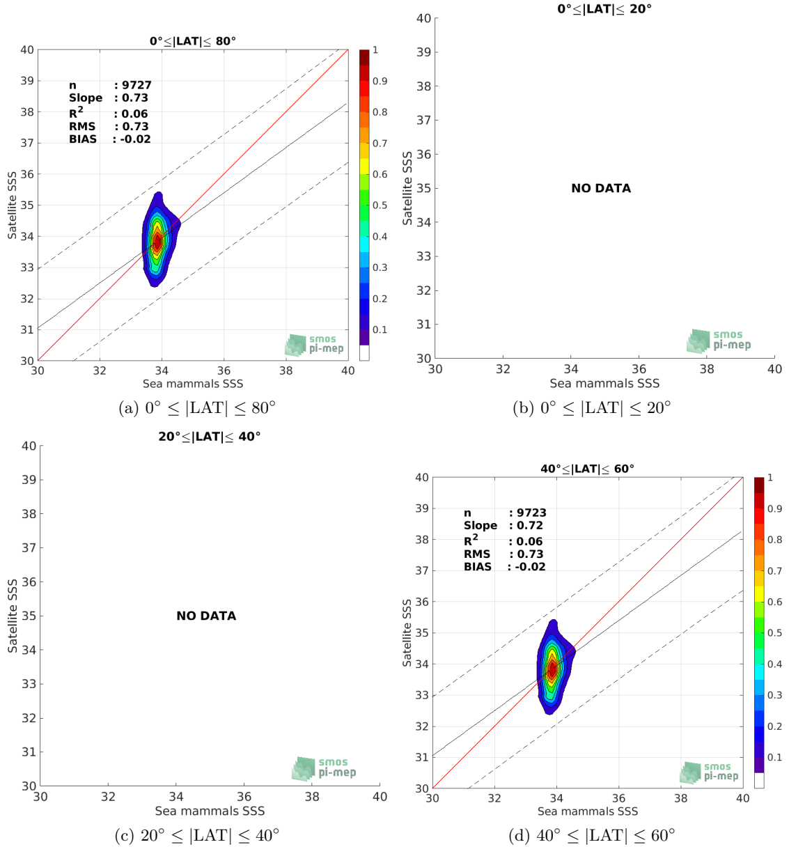
Figure 9: Contour maps of the concentration of SMOS SSS L3 v3 Monthly (ICDC) SSS (y-axis) versus Sea mammals SSS (x-axis) at match-up pairs for different latitude bands. For each plot, the red line shows x=y . The black thin and dashed lines indicate a linear fit through the data cloud and the \pm 95\% confidence levels, respectively. The number match-up pairs n , the slope and R^2 coefficient of the linear fit, the root mean square (RMS) and the mean bias between satellite and in situ data are indicated for each latitude band in each plots.
