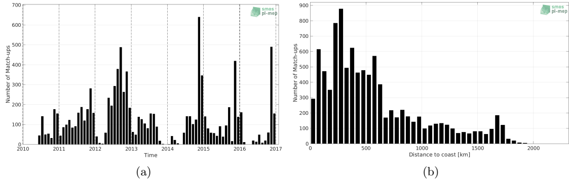
Figure 1: Number of match-ups between Sea mammals and SMOS SSS L3 v3 Monthly (ICDC) SSS as a function of time (a) and as function of the distance to coast (b) over the Indian Ocean Pi-MEP region and for the full satellite product period.
