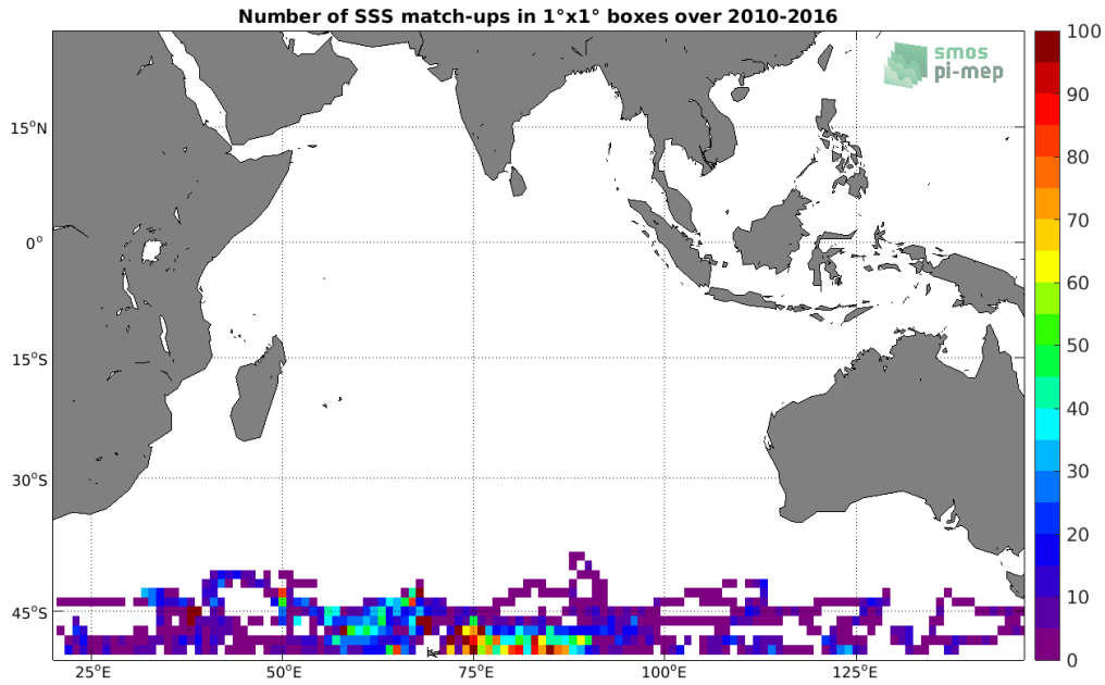
Figure 4: Number of SSS match-ups between Sea mammals SSS and the SMOS SSS L3 v3 Monthly (ICDC) SSS product for the Indian Ocean Pi-MEP region over 1°x1° boxes and for the full satellite product period.
