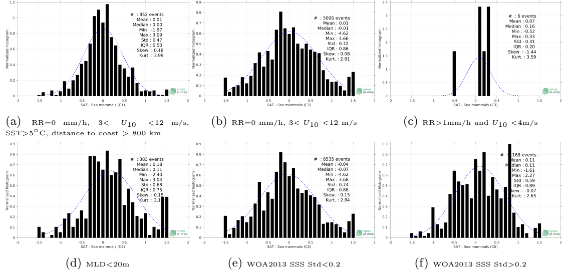
Figure 13: Normalized histogram of \Delta SSS (SMOS SSS L3 v3 Monthly (ICDC) - Sea mammals) for 6 different subdatasets corresponding to: RR=0 mm/h, 3 < U_{10} < 12 m/s, SST>5°C, distance to coast > 800 km (a), RR=0 mm/h, 3 < U_{10} < 12 m/s (b), RR>1mm/h and U_{10} < 4 m/s (c), MLD<20m (d), WOA2013 SSS Std<0.2 (e), WOA2013 SSS Std>0.2 (f).
