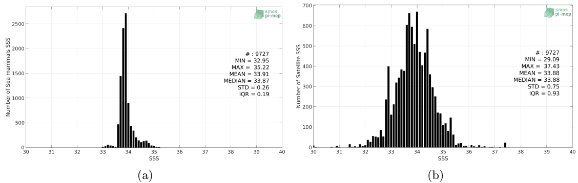
Figure 2: Histograms of SSS from Sea mammals (a) and SMOS-L3-ICDC-V3-MONTHLY-0.5DEG (b) considering all match-up pairs per bins of 0.1 over the Indian Ocean Pi-MEP region and for the full satellite product period.
