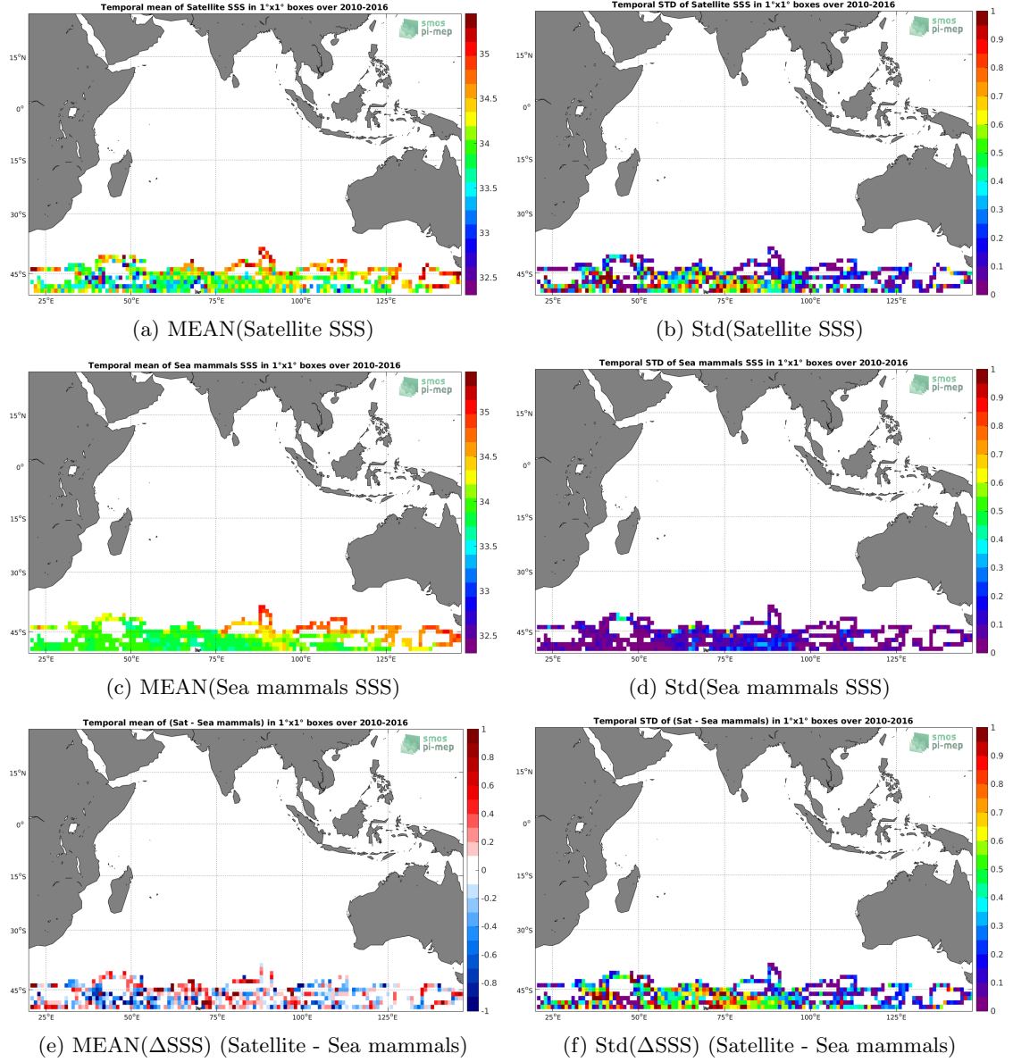
Figure 6: Temporal mean (left) and Std (right) of SSS from SMOS-L3-ICDC-V3-MONTHLY-0.5DEG (top), Sea mammals (middle), and of \Delta SSS (Satellite - Sea mammals). Only match-up pairs are used to generate these maps.
