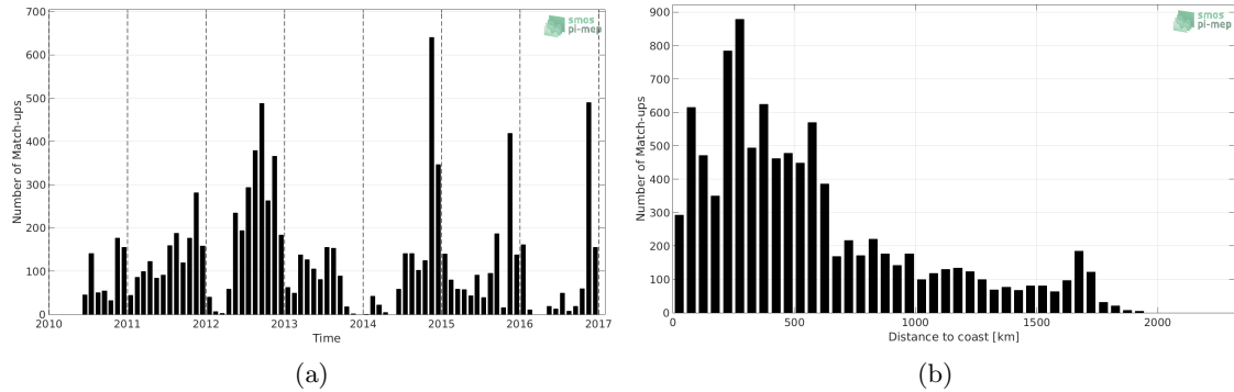
Figure 1: Number of match-ups between Sea mammals and SMOS-L3-ICDC-V3-MONTHLY-0.5DEG SSS as a function of time (a) and as function of the distance to coast (b) over the Indian Ocean Pi-MEP region and for the full satellite product period.
