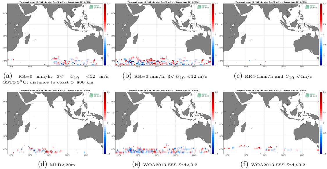
Figure 12: Temporal mean gridded over spatial boxes of size 1^{\circ}\times 1^{\circ} of \Delta\text{SSS} (SMOS-L3-ICDC-V3-MONTHLY-0.5DEG - Sea mammals) for 6 different subdatasets corresponding to: \text{RR}=0 mm/h, 3 < U_{10} < 12 m/s, \text{SST} > 5^{\circ}\text{C} , distance to coast > 800 km (a), \text{RR}=0 mm/h, 3 < U_{10} < 12 m/s (b), \text{RR} > 1\text{mm/h} and U_{10} < 4\text{m/s} (c), \text{MLD} < 20\text{m} (d), \text{WOA2013 SSS Std} < 0.2 (e), \text{WOA2013 SSS Std} > 0.2 (f).
