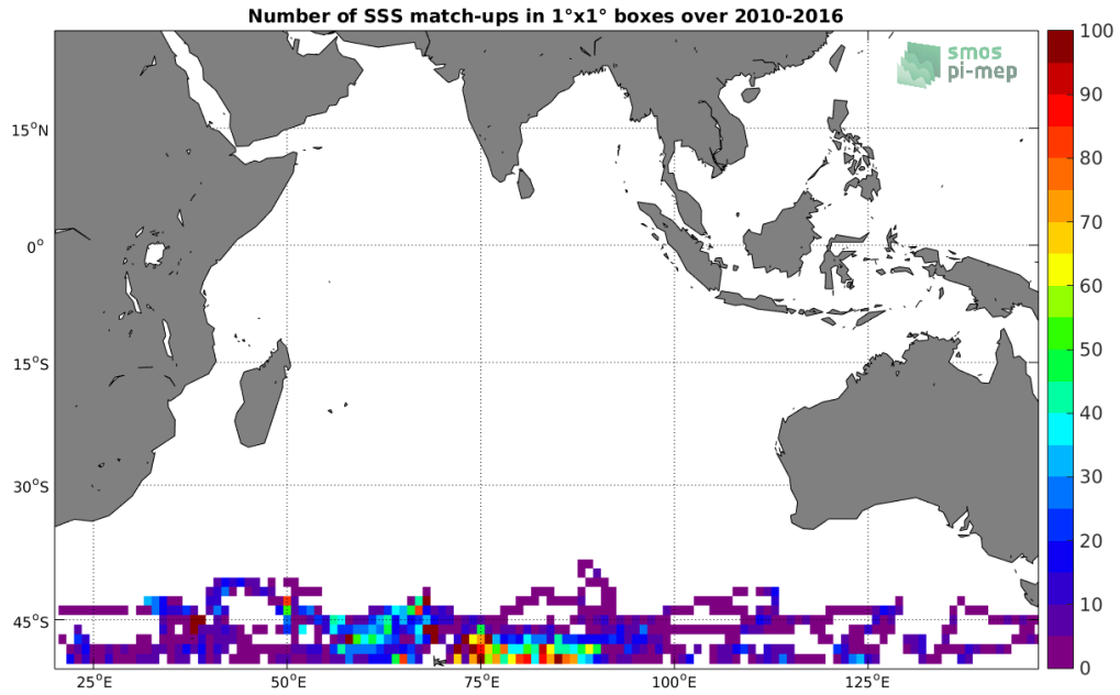
Figure 4: Number of SSS match-ups between Sea mammals SSS and the SMOS-L3-ICDC-V3-MONTHLY-0.5DEG SSS product for the Indian Ocean Pi-MEP region over 1°x1° boxes and for the full satellite product period.
