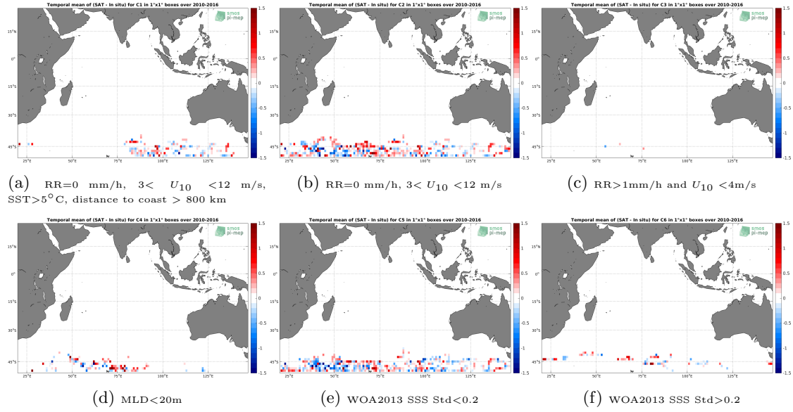
Figure 12: Temporal mean gridded over spatial boxes of size 1^\circ \times 1^\circ of \Delta SSS (SMOS-L3-ICDC-V3-MONTHLY-0.5DEG - Sea mammals) for 6 different subdatasets corresponding to: RR=0 mm/h, 3 < U_{10} < 12 m/s, SST > 5^\circ C , distance to coast > 800 km (a), RR=0 mm/h, 3 < U_{10} < 12 m/s (b), RR > 1 mm/h and U_{10} < 4 m/s (c), MLD < 20 m (d), WOA2013 SSS Std < 0.2 (e), WOA2013 SSS Std > 0.2 (f).
