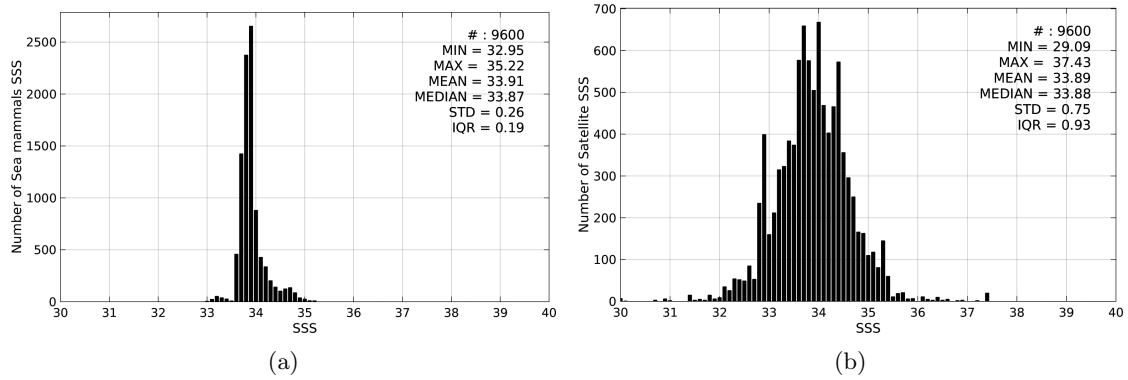
Figure 2: Histograms of SSS from Sea mammals (a) and SMOS-L3-ICDC-V3-MONTHLY-0.5DEG (b) considering all match-up pairs per bins of 0.1 over the Indian Ocean Pi-MEP region and for the full satellite product period.
