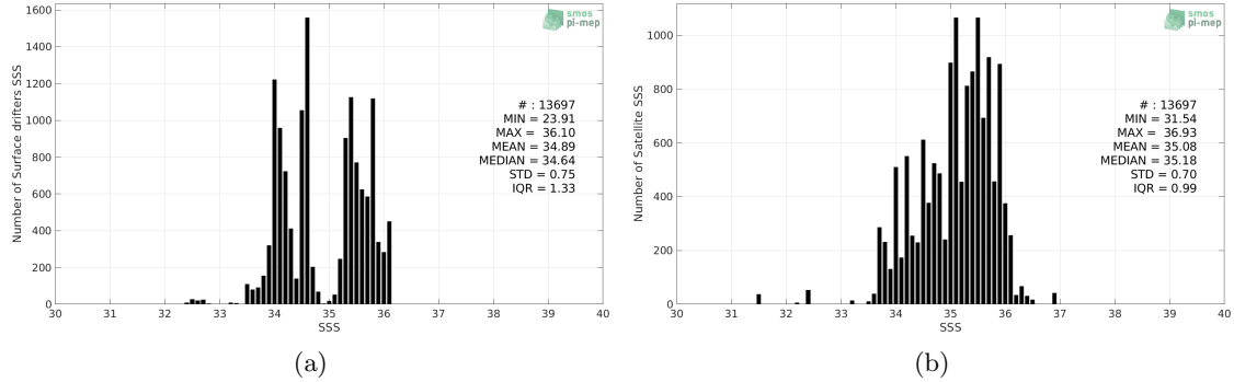
Figure 2: Histograms of SSS from Surface drifters (a) and SMOS SSS L3 v3 Monthly (ICDC) (b) considering all match-up pairs per bins of 0.1 over the Indian Ocean Pi-MEP region and for the full satellite product period.
