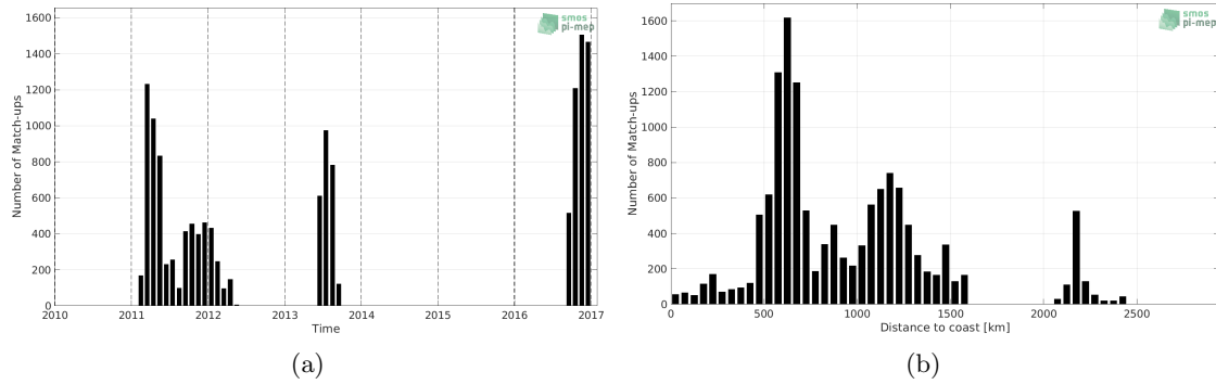
Figure 1: Number of match-ups between Surface drifters and SMOS SSS L3 v3 Monthly (ICDC) SSS as a function of time (a) and as function of the distance to coast (b) over the Indian Ocean Pi-MEP region and for the full satellite product period.
