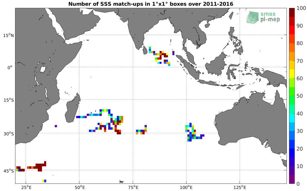
Figure 3: Number of SSS match-ups between Surface drifters SSS and the SMOS SSS L3 v3 Monthly (ICDC) SSS product for the Indian Ocean Pi-MEP region over 1^\circ \times 1^\circ boxes and for the full satellite product period.
