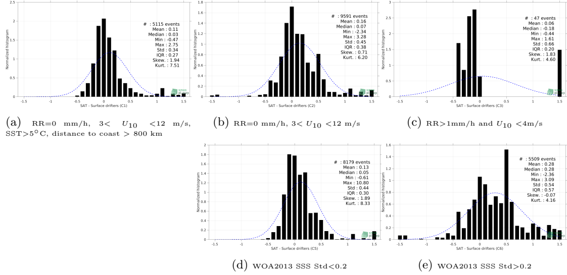
Figure 12: Normalized histogram of \Delta SSS (SMOS SSS L3 v3 Monthly (ICDC) - Surface drifters) for 5 different subdatasets corresponding to: RR=0 mm/h, 3 < U_{10} < 12 m/s, SST>5°C, distance to coast > 800 km (a), RR=0 mm/h, 3 < U_{10} < 12 m/s (b), RR>1mm/h and U_{10} < 4 m/s (c), WOA2013 SSS Std<0.2 (d), WOA2013 SSS Std>0.2 (e).
