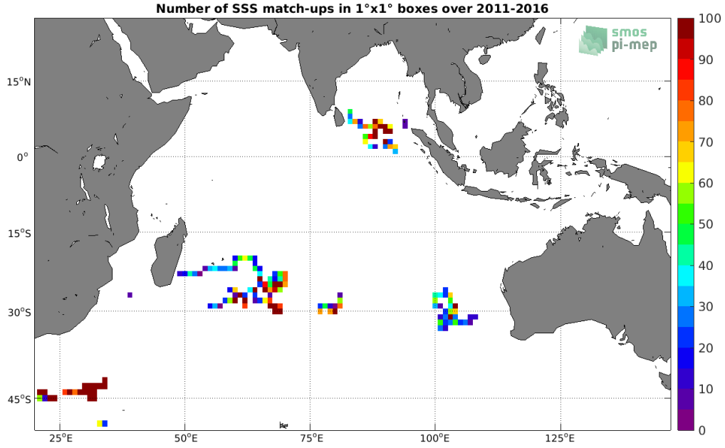
Figure 3: Number of SSS match-ups between Surface drifters SSS and the SMOS SSS L3 v3 Monthly (ICDC) SSS product for the Indian Ocean Pi-MEP region over 1^\circ \times 1^\circ boxes and for the full satellite product period.
