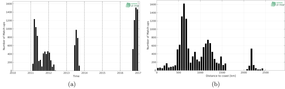
Figure 1: Number of match-ups between Surface drifters and SMOS-L3-ICDC-V3-MONTHLY-0.5DEG SSS as a function of time (a) and as function of the distance to coast (b) over the Indian Ocean Pi-MEP region and for the full satellite product period.
