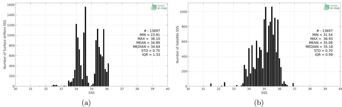
Figure 2: Histograms of SSS from Surface drifters (a) and SMOS-L3-ICDC-V3-MONTHLY-0.5DEG (b) considering all match-up pairs per bins of 0.1 over the Indian Ocean Pi-MEP region and for the full satellite product period.
