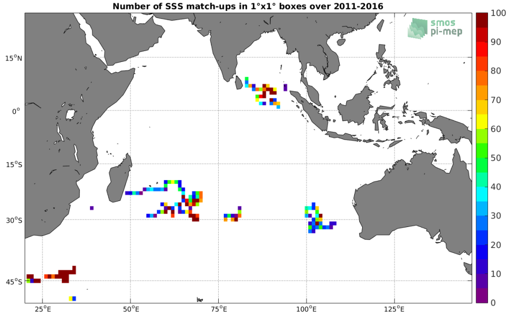
Figure 3: Number of SSS match-ups between Surface drifters SSS and the SMOS-L3-ICDC-V3-MONTHLY-0.5DEG SSS product for the Indian Ocean Pi-MEP region over 1^\circ \times 1^\circ boxes and for the full satellite product period.
