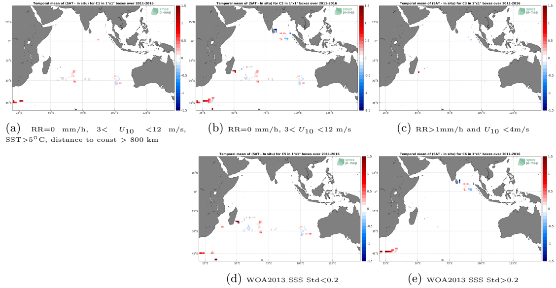
Figure 11: Temporal mean gridded over spatial boxes of size 1^\circ \times 1^\circ of \Delta SSS (SMOS-L3-ICDC-V3-MONTHLY-0.5DEG - Surface drifters) for 5 different subdatasets corresponding to: RR=0 mm/h, 3 < U_{10} < 12 m/s, SST > 5^\circ C , distance to coast > 800 km (a), RR=0 mm/h, 3 < U_{10} < 12 m/s (b), RR > 1 mm/h and U_{10} < 4 m/s (c), WOA2013 SSS Std < 0.2 (d), WOA2013 SSS Std > 0.2 (e).
