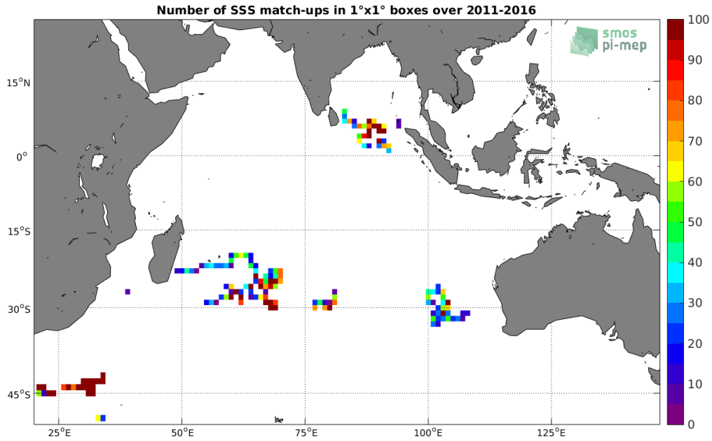
Figure 3: Number of SSS match-ups between Surface drifters SSS and the SMOS-L3-ICDC-V3-MONTHLY-0.5DEG SSS product for the Indian Ocean Pi-MEP region over 1°x1° boxes and for the full satellite product period.
