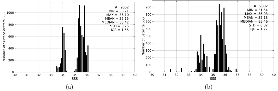
Figure 2: Histograms of SSS from Surface drifters (a) and SMOS-L3-ICDC-V3-MONTHLY-0.5DEG (b) considering all match-up pairs per bins of 0.1 over the Indian Ocean Pi-MEP region and for the full satellite product period.
