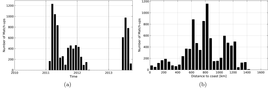
Figure 1: Number of match-ups between Surface drifters and SMOS-L3-ICDC-V3-MONTHLY-0.5DEG SSS as a function of time (a) and as function of the distance to coast (b) over the Indian Ocean Pi-MEP region and for the full satellite product period.
