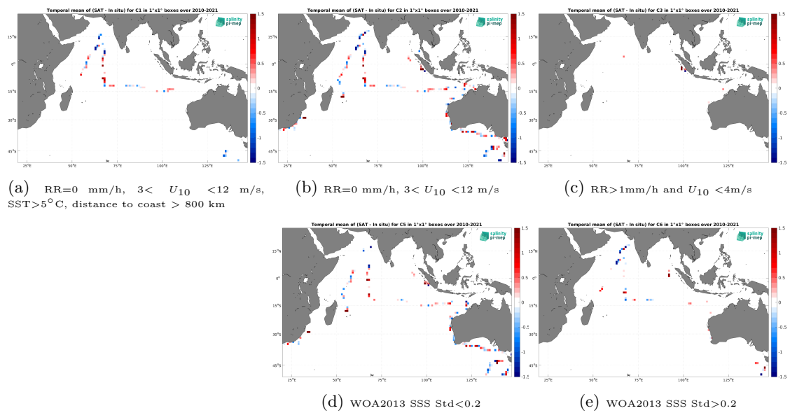
Figure 14: Temporal mean gridded over spatial boxes of size 1^\circ \times 1^\circ of \Delta SSS (SMOS SSS L2Q v331 - With FLAG (CMEMS-CATDS-CPDC) - TSG (SAMOS)) for 5 different subdatasets corresponding to:RR=0 mm/h, 3 < U_{10} < 12 m/s, SST >5^\circ\text{C} , distance to coast > 800 km (a), RR=0 mm/h, 3 < U_{10} < 12 m/s (b), RR >1 mm/h and U_{10} < 4 m/s (c), WOA2013 SSS Std <0.2 (d), WOA2013 SSS Std >0.2 (e).
