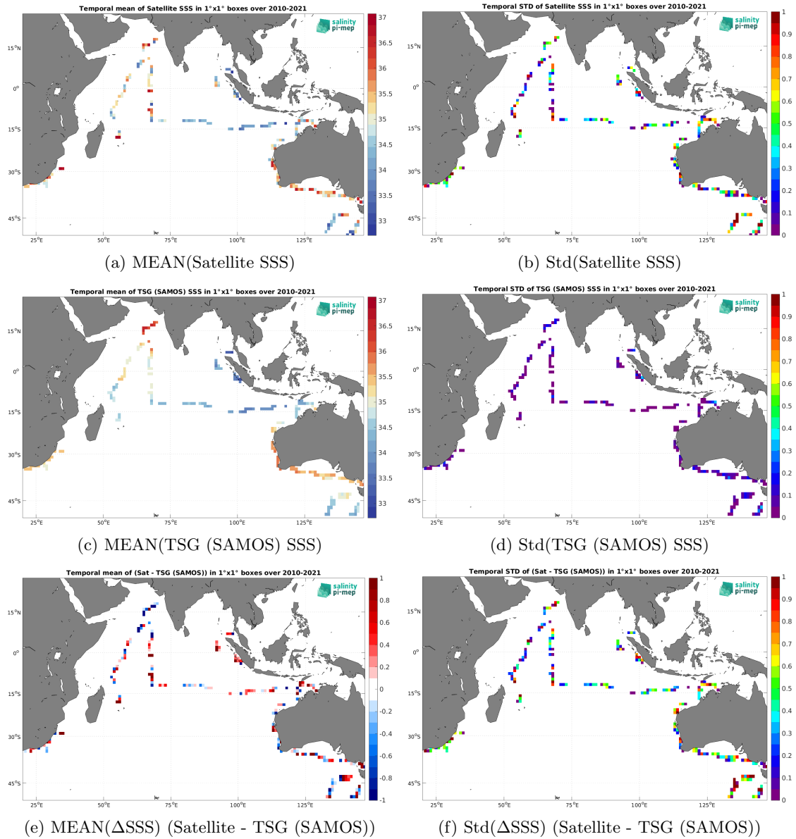
Figure 7: Temporal mean (left) and Std (right) of SSS from SMOS SSS L2Q v331 - With FLAG (CMEMS-CATDS-CPDC) (top), TSG (SAMOS) (middle), and of \Delta SSS (Satellite - TSG (SAMOS)). Only match-up pairs are used to generate these maps.
