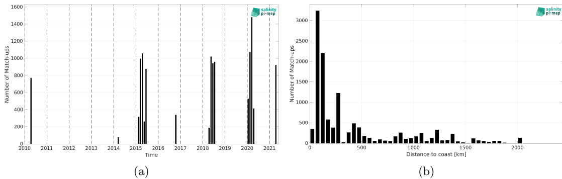
Figure 2: Number of match-ups between TSG (SAMOS) and SMOS SSS L2Q v331 - With FLAG (CMEMS-CATDS-CPDC) SSS as a function of time (a) and as function of the distance to coast (b) over the Indian Ocean Pi-MEP region and for the full satellite product period.
