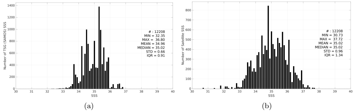
Figure 3: Histograms of SSS from TSG (SAMOS) (a) and SMOS SSS L2Q v331 - With FLAG (CMEMS-CATDS-CPDC) (b) considering all match-up pairs per bins of 0.1 over the Indian Ocean Pi-MEP region and for the full satellite product period.
