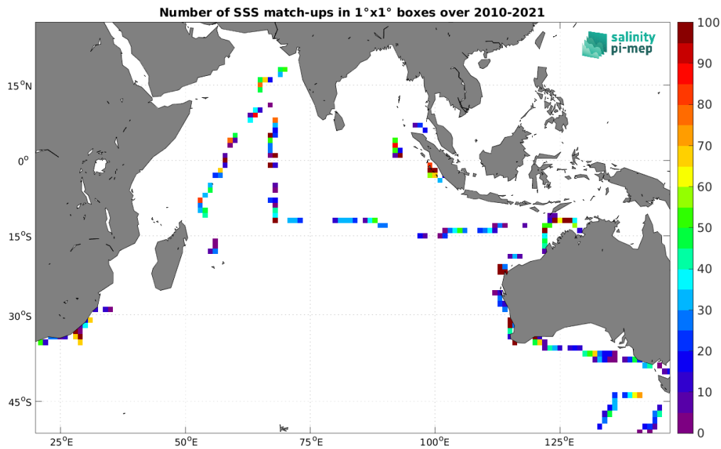
Figure 4: Number of SSS match-ups between TSG (SAMOS) SSS and the SMOS SSS L2Q v331 - With FLAG (CMEMS-CATDS-CPDC) SSS product for the Indian Ocean Pi-MEP region over 1^\circ \times 1^\circ boxes and for the full satellite product period.
