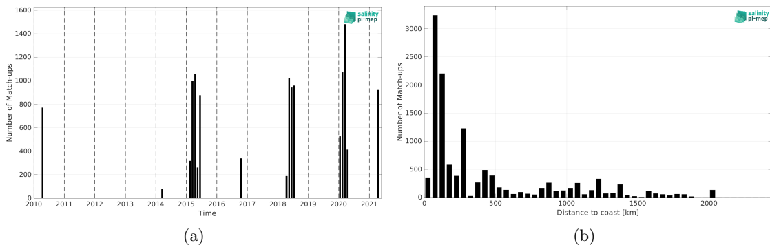
Figure 1: Number of match-ups between TSG (SAMOS) and SMOS SSS L2Q v331 - With FLAG (CMEMS-CATDS-CPDC) SSS as a function of time (a) and as function of the distance to coast (b) over the Indian Ocean Pi-MEP region and for the full satellite product period.
