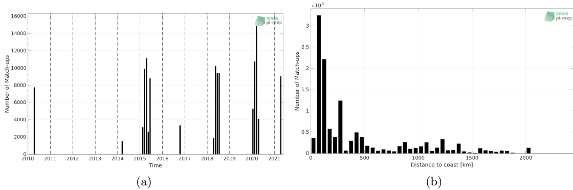
Figure 1: Number of match-ups between TSG (SAMOS) and SMOS SSS L2Q v331 - With FLAG (CMEMS-CATDS-CPDC) SSS as a function of time (a) and as function of the distance to coast (b) over the Indian Ocean Pi-MEP region and for the full satellite product period.
