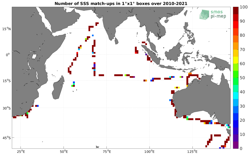
Figure 4: Number of SSS match-ups between TSG (SAMOS) SSS and the SMOS SSS L2Q v331 - With FLAG (CMEMS-CATDS-CPDC) SSS product for the Indian Ocean Pi-MEP region over 1^\circ \times 1^\circ boxes and for the full satellite product period.
