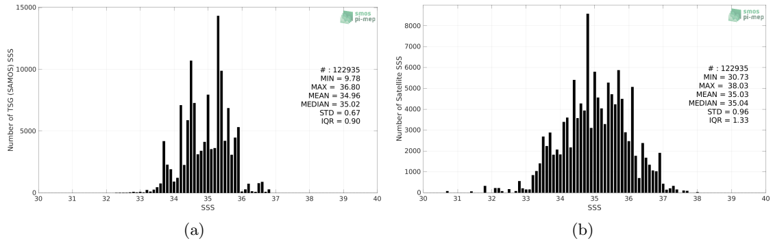
Figure 2: Histograms of SSS from TSG (SAMOS) (a) and SMOS SSS L2Q v331 - With FLAG (CMEMS-CATDS-CPDC) (b) considering all match-up pairs per bins of 0.1 over the Indian Ocean Pi-MEP region and for the full satellite product period.
