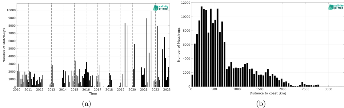
Figure 2: Number of match-ups between TSG (LEGOS-DM) and SMOS SSS L2Q v331 - With FLAG (CMEMS-CATDS-CPDC) SSS as a function of time (a) and as function of the distance to coast (b) over the Indian Ocean Pi-MEP region and for the full satellite product period.
