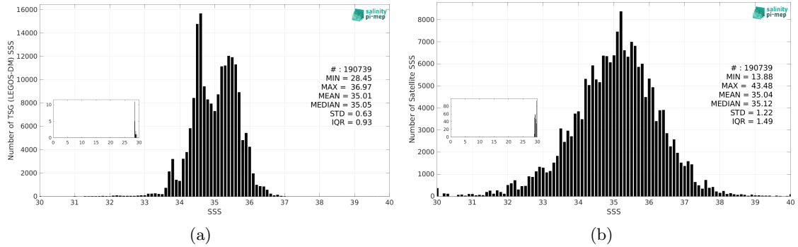
Figure 3: Histograms of SSS from TSG (LEGOS-DM) (a) and SMOS SSS L2Q v331 - With FLAG (CMEMS-CATDS-CPDC) (b) considering all match-up pairs per bins of 0.1 over the Indian Ocean Pi-MEP region and for the full satellite product period.
