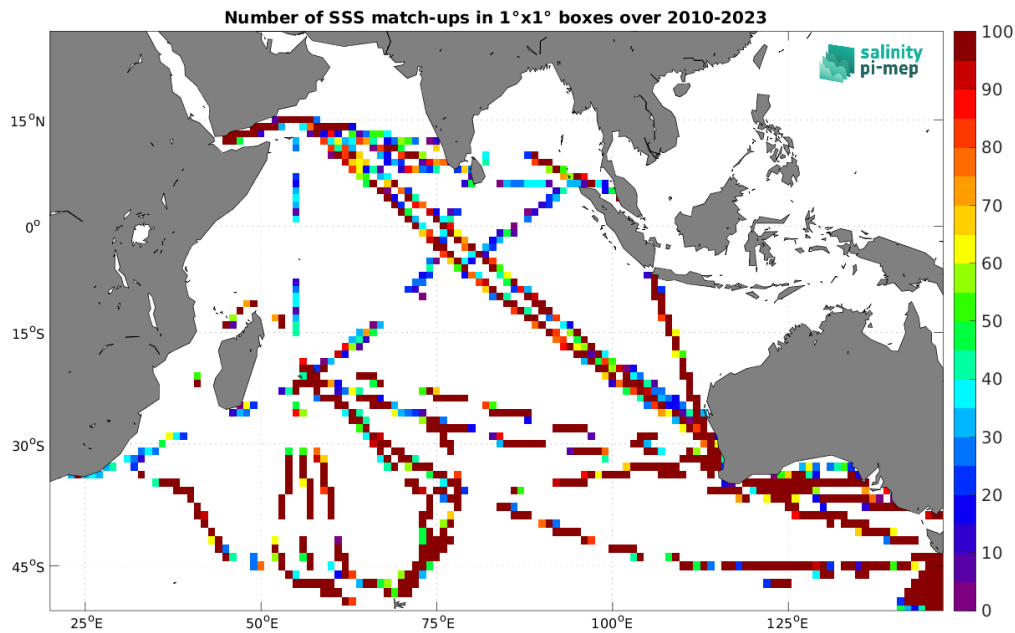
Figure 5: Number of SSS match-ups between TSG (LEGOS-DM) SSS and the SMOS SSS L2Q v331 - With FLAG (CMEMS-CATDS-CPDC) SSS product for the Indian Ocean Pi-MEP region over 1^\circ \times 1^\circ boxes and for the full satellite product period.
