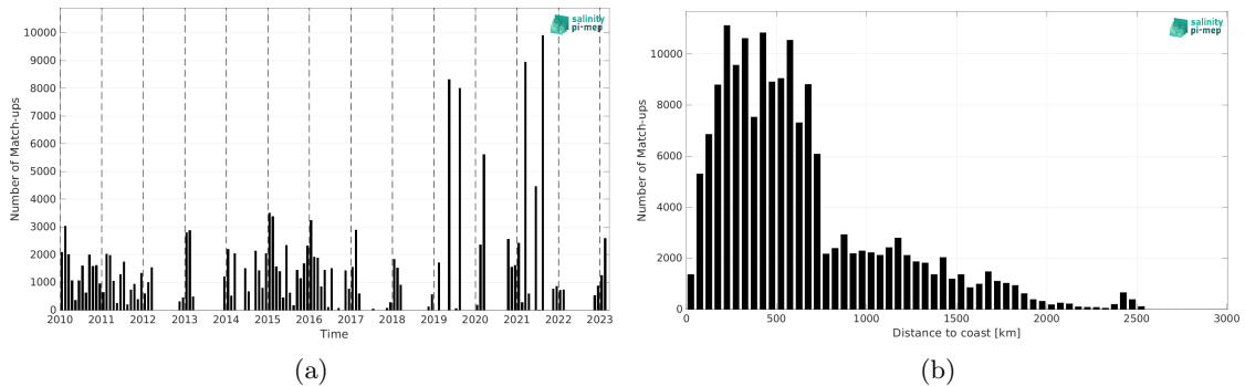
Figure 1: Number of match-ups between TSG (LEGOS-DM) and SMOS SSS L2Q v331 - With FLAG (CMEMS-CATDS-CPDC) SSS as a function of time (a) and as function of the distance to coast (b) over the Indian Ocean Pi-MEP region and for the full satellite product period.
