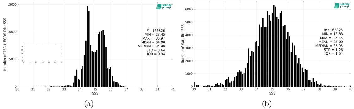
Figure 2: Histograms of SSS from TSG (LEGOS-DM) (a) and SMOS SSS L2Q v331 - With FLAG (CMEMS-CATDS-CPDC) (b) considering all match-up pairs per bins of 0.1 over the Indian Ocean Pi-MEP region and for the full satellite product period.
