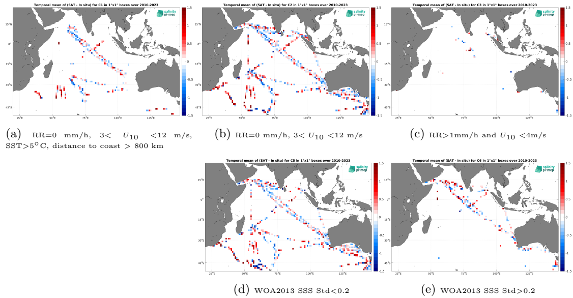
Figure 12: Temporal mean gridded over spatial boxes of size 1^\circ \times 1^\circ of \Delta SSS (SMOS SSS L2Q v331 - With FLAG (CMEMS-CATDS-CPDC) - TSG (LEGOS-DM)) for 5 different subdatasets corresponding to:RR=0 mm/h, 3 < U_{10} < 12 m/s, SST >5^\circ C, distance to coast > 800 km (a), RR=0 mm/h, 3 < U_{10} < 12 m/s (b), RR >1 mm/h and U_{10} < 4 m/s (c), WOA2013 SSS Std <0.2 (d), WOA2013 SSS Std >0.2 (e).
