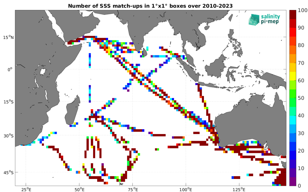
Figure 4: Number of SSS match-ups between TSG (LEGOS-DM) SSS and the SMOS SSS L2Q v331 - With FLAG (CMEMS-CATDS-CPDC) SSS product for the Indian Ocean Pi-MEP region over 1^\circ \times 1^\circ boxes and for the full satellite product period.
