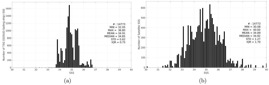
Figure 3: Histograms of SSS from TSG (GOSUD-Sailing-ship) (a) and SMOS SSS L2Q v331 - With FLAG (CMEMS-CATDS-CPDC) (b) considering all match-up pairs per bins of 0.1 over the Indian Ocean Pi-MEP region and for the full satellite product period.
