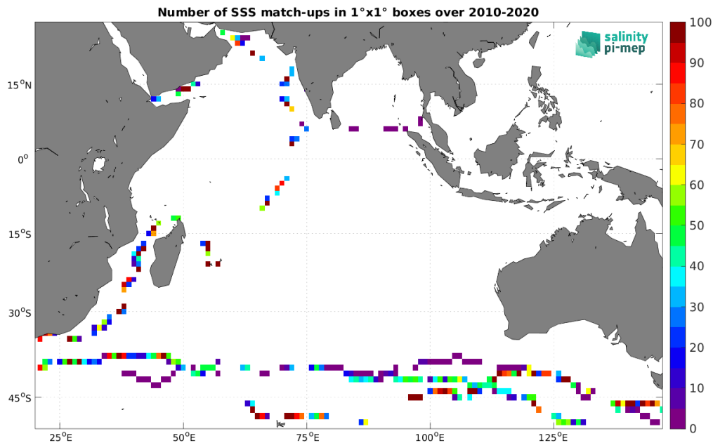
Figure 5: Number of SSS match-ups between TSG (GOSUD-Sailing-ship) SSS and the SMOS SSS L2Q v331 - With FLAG (CMEMS-CATDS-CPDC) SSS product for the Indian Ocean Pi-MEP region over 1^{\circ} \times 1^{\circ} boxes and for the full satellite product period.
