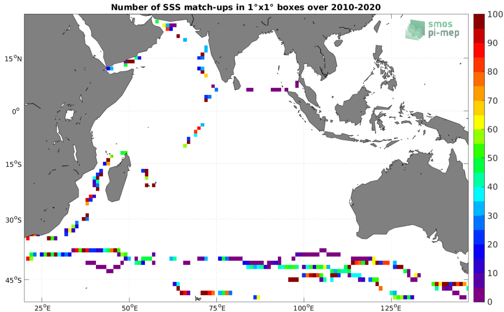
Figure 4: Number of SSS match-ups between TSG (GOSUD-Sailing-ship) SSS and the SMOS SSS L2Q v331 - With FLAG (CMEMS-CATDS-CPDC) SSS product for the Indian Ocean Pi-MEP region over 1^\circ \times 1^\circ boxes and for the full satellite product period.
