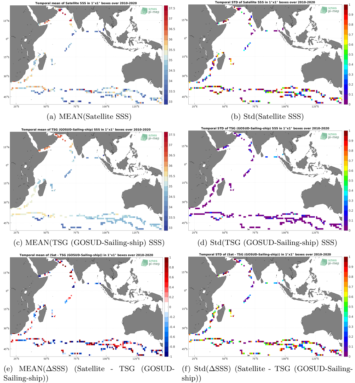
Figure 6: Temporal mean (left) and Std (right) of SSS from SMOS SSS L2Q v331 - With FLAG (CMEMS-CATDS-CPDC) (top), TSG (GOSUD-Sailing-ship) (middle), and of \Delta SSS (Satellite - TSG (GOSUD-Sailing-ship)). Only match-up pairs are used to generate these maps.
