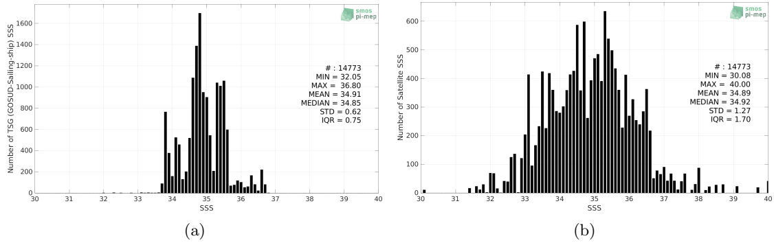
Figure 2: Histograms of SSS from TSG (GOSUD-Sailing-ship) (a) and SMOS SSS L2Q v331 - With FLAG (CMEMS-CATDS-CPDC) (b) considering all match-up pairs per bins of 0.1 over the Indian Ocean Pi-MEP region and for the full satellite product period.
