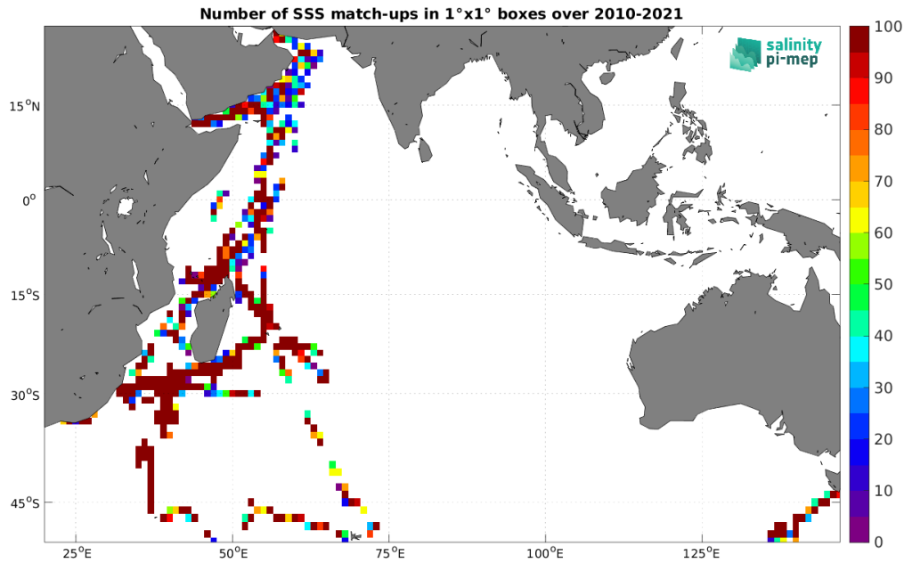
Figure 4: Number of SSS match-ups between TSG (GOSUD-Research-vessel) SSS and the SMOS SSS L2Q v331 - With FLAG (CMEMS-CATDS-CPDC) SSS product for the Indian Ocean Pi-MEP region over 1^\circ \times 1^\circ boxes and for the full satellite product period.
