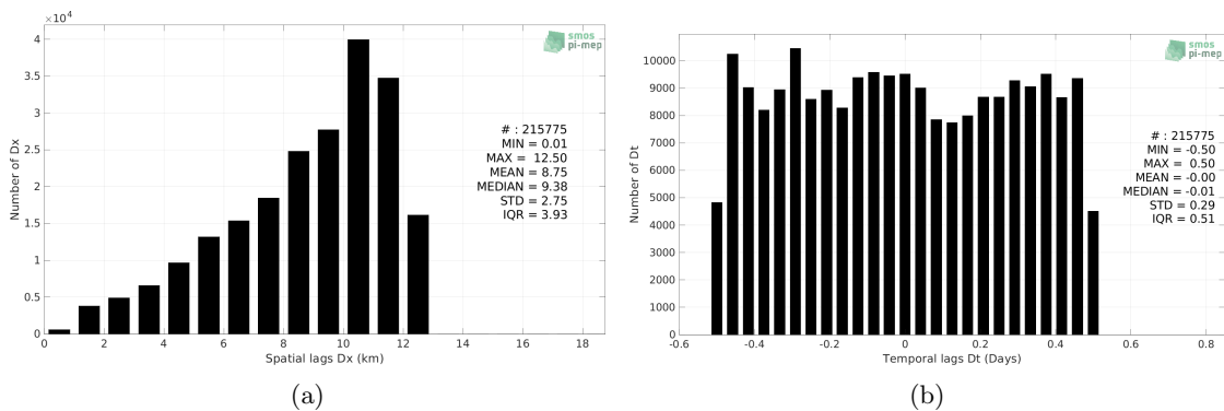
Figure 5: Histograms of the spatial (a) and temporal (b) lags between the location/time of the TSG (GOSUD-Research-vessel) measurement and the date of the corresponding SMOS SSS L2Q v331 - With FLAG (CMEMS-CATDS-CPDC) SSS pixel.
