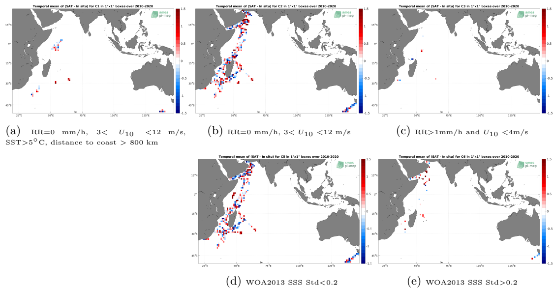
Figure 12: Temporal mean gridded over spatial boxes of size 1^\circ \times 1^\circ of \Delta SSS (SMOS SSS L2Q v331 - With FLAG (CMEMS-CATDS-CPDC) - TSG (GOSUD-Research-vessel)) for 5 different subdatasets corresponding to:RR=0 mm/h, 3 < U_{10} < 12 m/s, SST > 5^\circ\text{C} , distance to coast > 800 km (a), RR=0 mm/h, 3 < U_{10} < 12 m/s (b), RR > 1 mm/h and U_{10} < 4 m/s (c), WOA2013 SSS Std < 0.2 (d), WOA2013 SSS Std > 0.2 (e).
