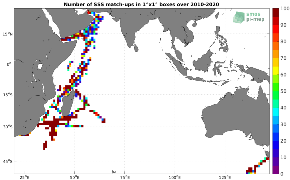
Figure 4: Number of SSS match-ups between TSG (GOSUD-Research-vessel) SSS and the SMOS SSS L2Q v331 - With FLAG (CMEMS-CATDS-CPDC) SSS product for the Indian Ocean Pi-MEP region over 1^\circ \times 1^\circ boxes and for the full satellite product period.
