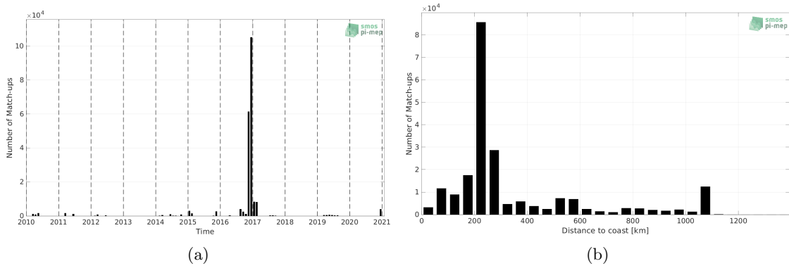
Figure 1: Number of match-ups between TSG (GOSUD-Research-vessel) and SMOS SSS L2Q v331 - With FLAG (CMEMS-CATDS-CPDC) SSS as a function of time (a) and as function of the distance to coast (b) over the Indian Ocean Pi-MEP region and for the full satellite product period.
