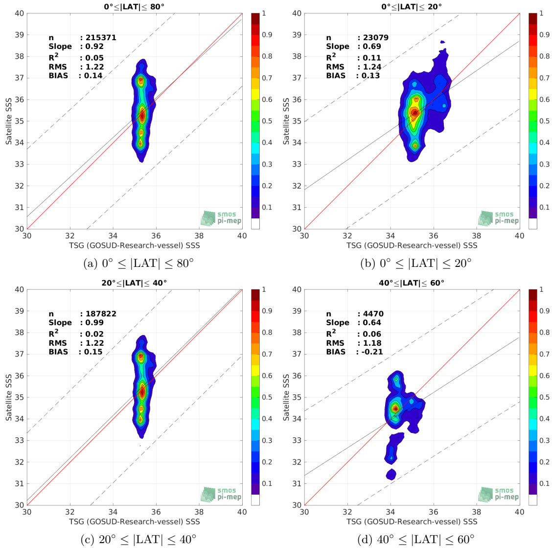
Figure 9: Contour maps of the concentration of SMOS SSS L2Q v331 - With FLAG (CMEMS-CATDS-CPDC) SSS ( y -axis) versus TSG (GOSUD-Research-vessel) SSS ( x -axis) at match-up pairs for different latitude bands. For each plot, the red line shows x=y . The black thin and dashed lines indicate a linear fit through the data cloud and the \pm 95\% confidence levels, respectively. The number match-up pairs n , the slope and R^2 coefficient of the linear fit, the root mean square (RMS) and the mean bias between satellite and in situ data are indicated for each latitude band in each plots.
