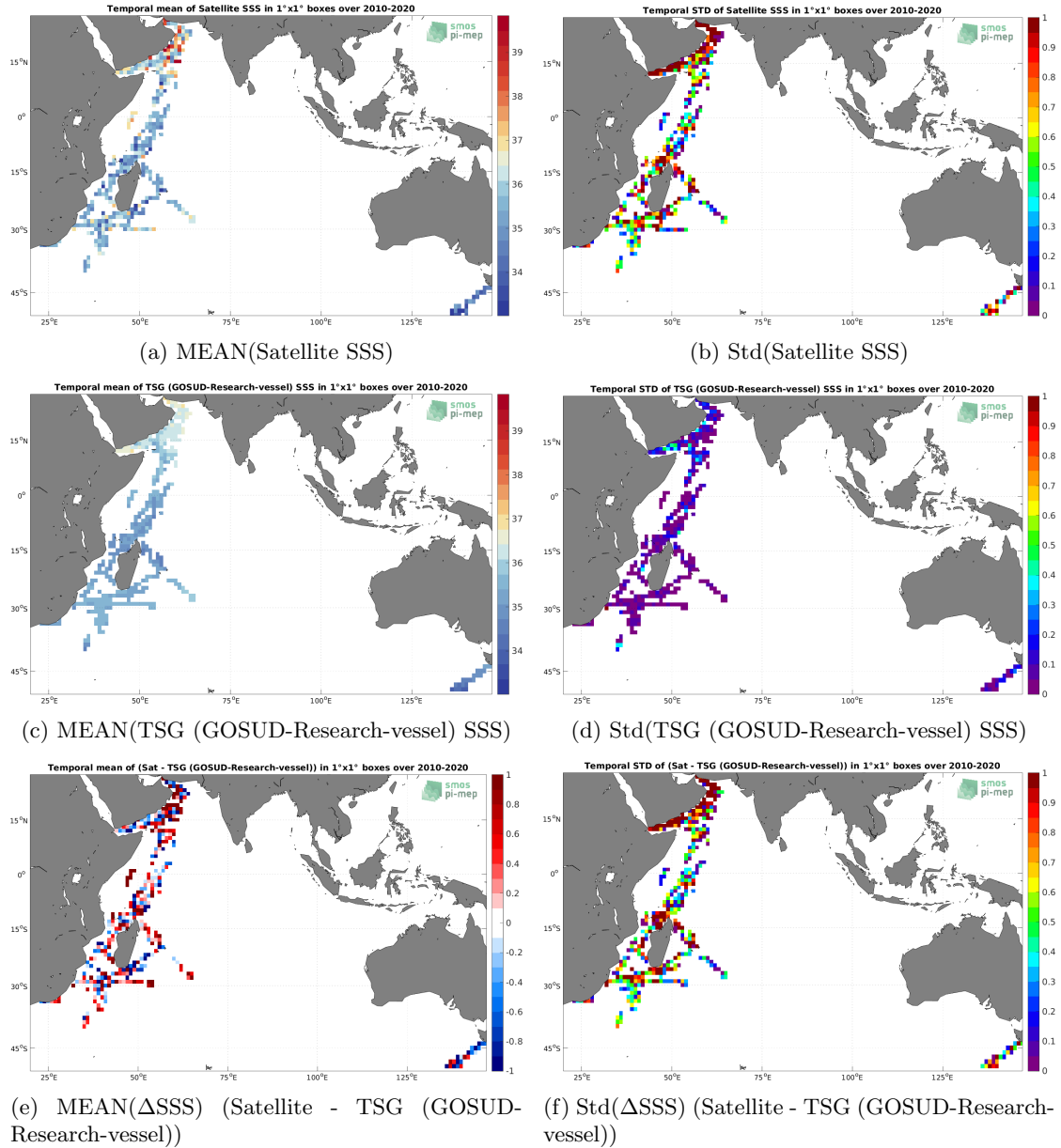
Figure 6: Temporal mean (left) and Std (right) of SSS from SMOS SSS L2Q v331 - With FLAG (CMEMS-CATDS-CPDC) (top), TSG (GOSUD-Research-vessel) (middle), and of \Delta SSS (Satellite - TSG (GOSUD-Research-vessel)). Only match-up pairs are used to generate these maps.
