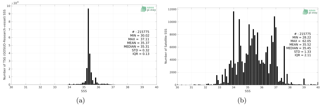
Figure 2: Histograms of SSS from TSG (GOSUD-Research-vessel) (a) and SMOS SSS L2Q v331 - With FLAG (CMEMS-CATDS-CPDC) (b) considering all match-up pairs per bins of 0.1 over the Indian Ocean Pi-MEP region and for the full satellite product period.
