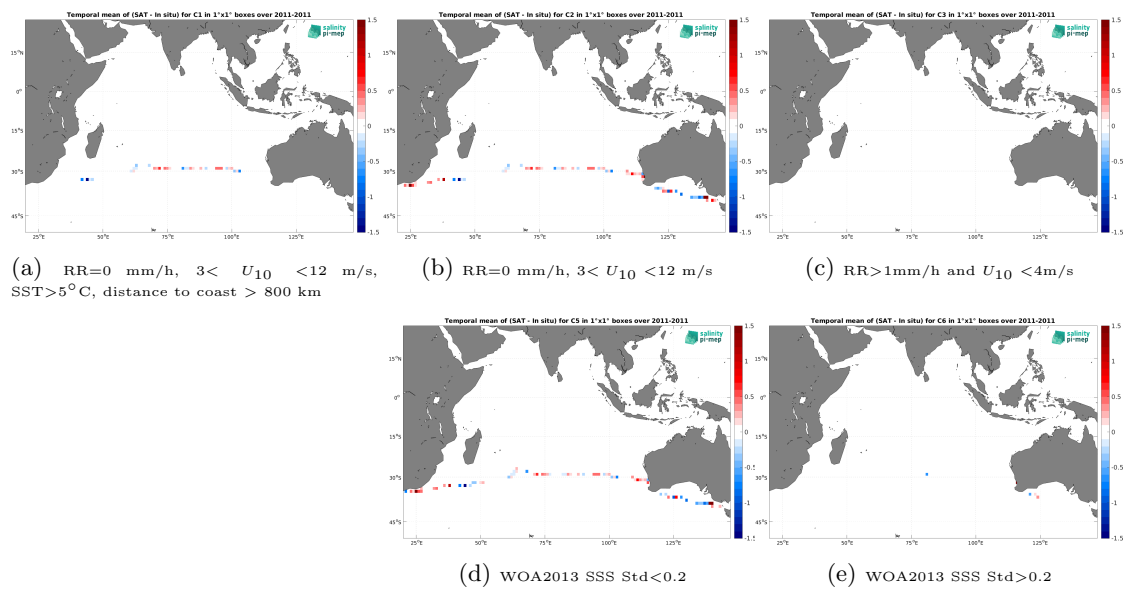
Figure 14: Temporal mean gridded over spatial boxes of size 1^\circ \times 1^\circ of \Delta SSS (SMOS SSS L2Q v331 - With FLAG (CMEMS-CATDS-CPDC) - TSG (CSIC-UTM)) for 5 different subdatasets corresponding to: RR=0 mm/h, 3 < U_{10} < 12 m/s, SST > 5^\circ\text{C} , distance to coast > 800 km (a), RR=0 mm/h, 3 < U_{10} < 12 m/s (b), RR > 1 mm/h and U_{10} < 4 m/s (c), WOA2013 SSS Std < 0.2 (d), WOA2013 SSS Std > 0.2 (e).
