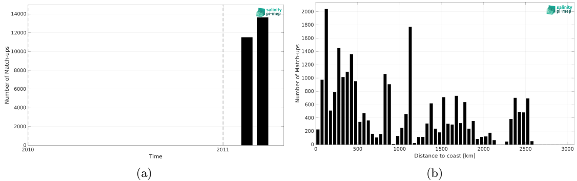
Figure 2: Number of match-ups between TSG (CSIC-UTM) and SMOS SSS L2Q v331 - With FLAG (CMEMS-CATDS-CPDC) SSS as a function of time (a) and as function of the distance to coast (b) over the Indian Ocean Pi-MEP region and for the full satellite product period.
