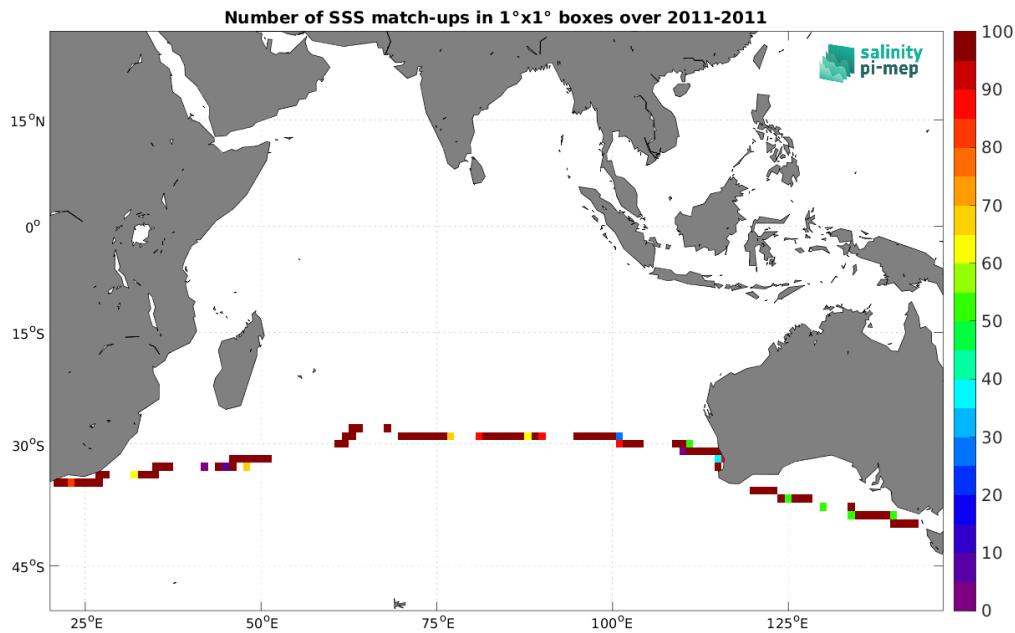
Figure 5: Number of SSS match-ups between TSG (CSIC-UTM) SSS and the SMOS SSS L2Q v331 - With FLAG (CMEMS-CATDS-CPDC) SSS product for the Indian Ocean Pi-MEP region over 1^\circ \times 1^\circ boxes and for the full satellite product period.
