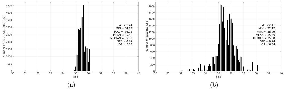
Figure 3: Histograms of SSS from TSG (CSIC-UTM) (a) and SMOS SSS L2Q v331 - With FLAG (CMEMS-CATDS-CPDC) (b) considering all match-up pairs per bins of 0.1 over the Indian Ocean Pi-MEP region and for the full satellite product period.
