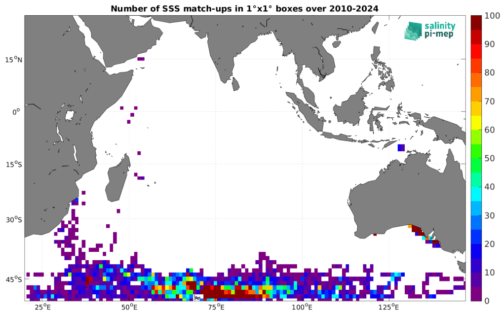
Figure 5: Number of SSS match-ups between Marine mammals SSS and the SMOS SSS L2Q v331 - With FLAG (CMEMS-CATDS-CPDC) SSS product for the Indian Ocean Pi-MEP region over 1^{\circ} \times 1^{\circ} boxes and for the full satellite product period.
