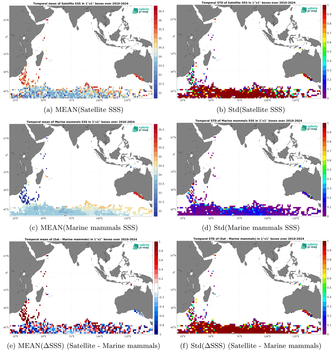
Figure 7: Temporal mean (left) and Std (right) of SSS from SMOS SSS L2Q v331 - With FLAG (CMEMS-CATDS-CPDC) (top), Marine mammals (middle), and of \Delta SSS (Satellite - Marine mammals). Only match-up pairs are used to generate these maps.
