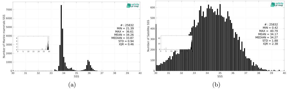
Figure 3: Histograms of SSS from Marine mammals (a) and SMOS SSS L2Q v331 - With FLAG (CMEMS-CATDS-CPDC) (b) considering all match-up pairs per bins of 0.1 over the Indian Ocean Pi-MEP region and for the full satellite product period.
