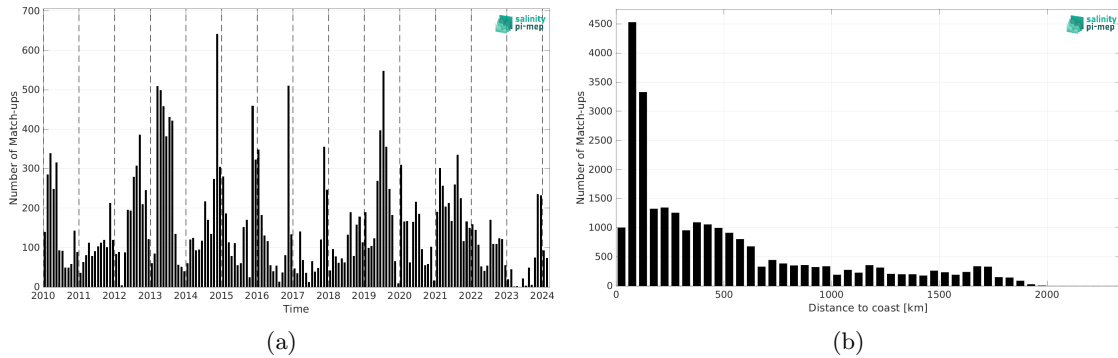
Figure 2: Number of match-ups between Marine mammals and SMOS SSS L2Q v331 - With FLAG (CMEMS-CATDS-CPDC) SSS as a function of time (a) and as function of the distance to coast (b) over the Indian Ocean Pi-MEP region and for the full satellite product period.
