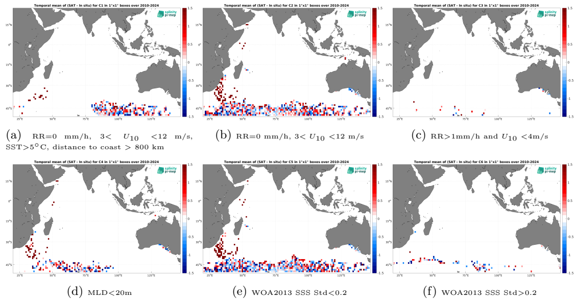
Figure 14: Temporal mean gridded over spatial boxes of size 1^\circ \times 1^\circ of \Delta\text{SSS} (SMOS SSS L2Q v331 - With FLAG (CMEMS-CATDS-CPDC) - Marine mammals) for 6 different subdatasets corresponding to:RR=0 mm/h, 3 < U_{10} < 12 m/s, SST>5°C, distance to coast > 800 km (a), RR=0 mm/h, 3 < U_{10} < 12 m/s (b), RR>1mm/h and U_{10} < 4 m/s (c),MLD<20m (d),WOA2013 SSS Std<0.2 (e),WOA2013 SSS Std>0.2 (f).
