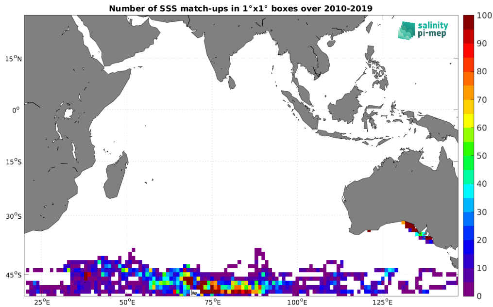
Figure 4: Number of SSS match-ups between Marine mammals SSS and the SMOS SSS L2Q v331 - With FLAG (CMEMS-CATDS-CPDC) SSS product for the Indian Ocean Pi-MEP region over 1^{\circ} \times 1^{\circ} boxes and for the full satellite product period.
