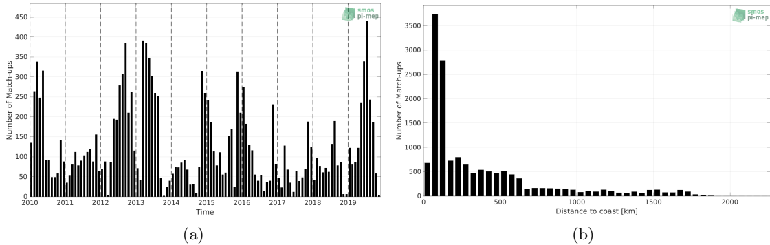
Figure 1: Number of match-ups between Marine mammals and SMOS SSS L2Q v331 - With FLAG (CMEMS-CATDS-CPDC) SSS as a function of time (a) and as function of the distance to coast (b) over the Indian Ocean Pi-MEP region and for the full satellite product period.
