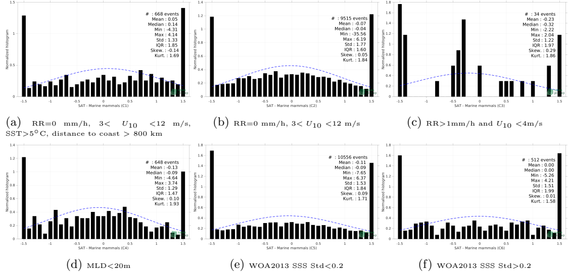
Figure 13: Normalized histogram of \Delta SSS (SMOS SSS L2Q v331 - With FLAG (CMEMS-CATDS-CPDC) - Marine mammals) for 6 different subdatasets corresponding to: RR=0 mm/h, 3 < U_{10} < 12 m/s, SST>5°C, distance to coast > 800 km (a), RR=0 mm/h, 3 < U_{10} < 12 m/s (b), RR>1mm/h and U_{10} < 4 m/s (c), MLD<20m (d), WOA2013 SSS Std<0.2 (e), WOA2013 SSS Std>0.2 (f).
