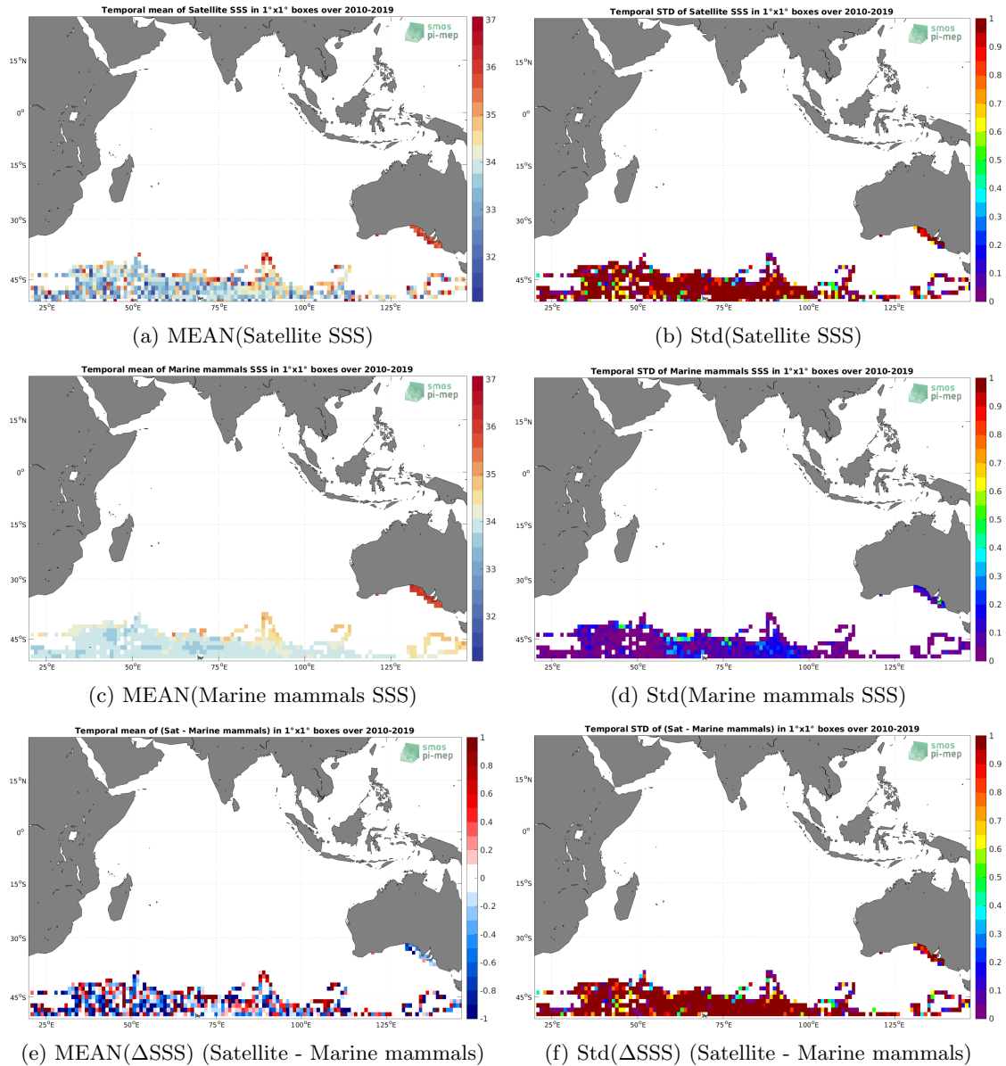
Figure 6: Temporal mean (left) and Std (right) of SSS from SMOS SSS L2Q v331 - With FLAG (CMEMS-CATDS-CPDC) (top), Marine mammals (middle), and of \Delta SSS (Satellite - Marine mammals). Only match-up pairs are used to generate these maps.
