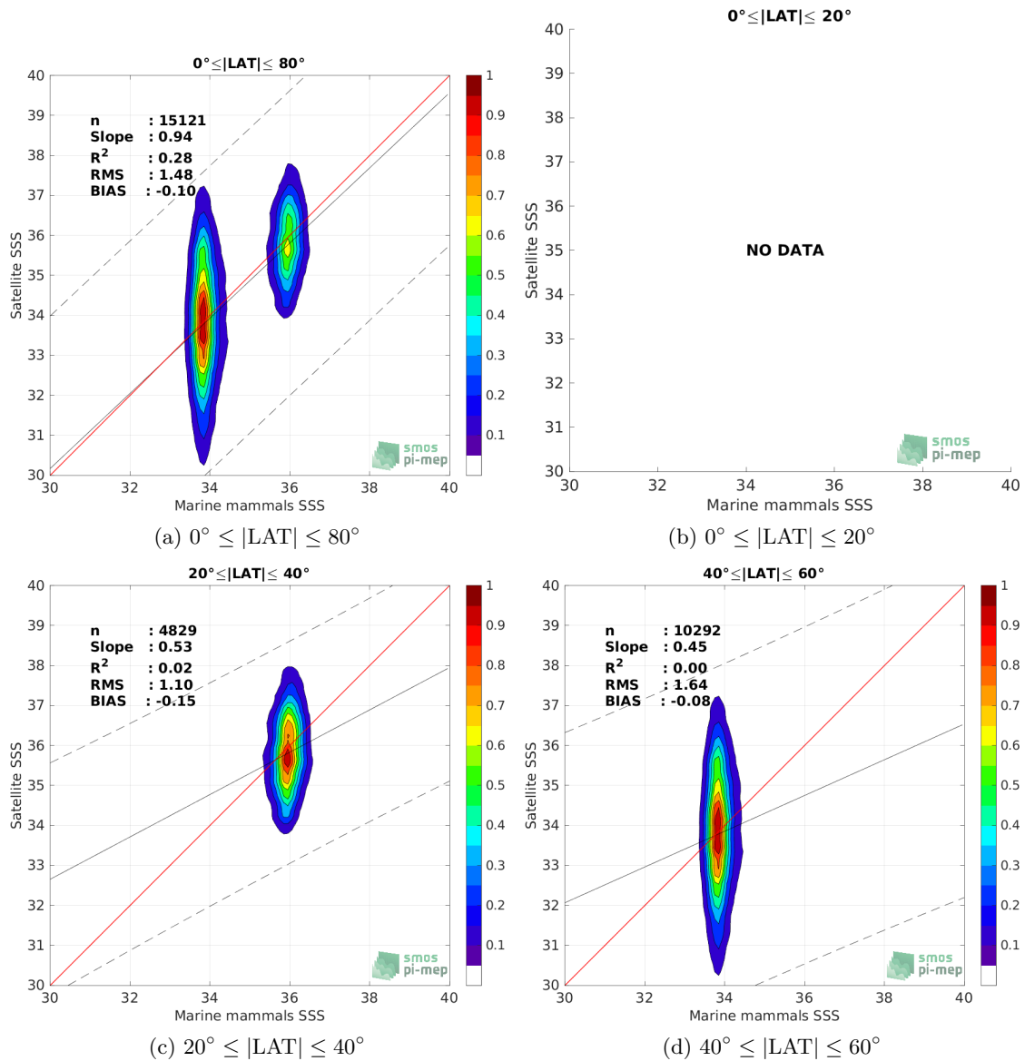
Figure 9: Contour maps of the concentration of SMOS SSS L2Q v331 - With FLAG (CMEMS-CATDS-CPDC) SSS (y-axis) versus Marine mammals SSS (x-axis) at match-up pairs for different latitude bands. For each plot, the red line shows x=y . The black thin and dashed lines indicate a linear fit through the data cloud and the \pm 95\% confidence levels, respectively. The number match-up pairs n , the slope and R^2 coefficient of the linear fit, the root mean square (RMS) and the mean bias between satellite and in situ data are indicated for each latitude band in each plots.
