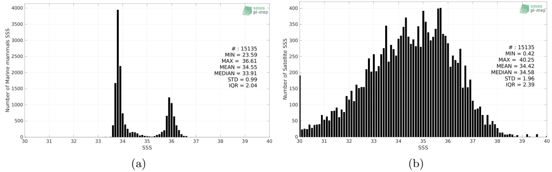
Figure 2: Histograms of SSS from Marine mammals (a) and SMOS SSS L2Q v331 - With FLAG (CMEMS-CATDS-CPDC) (b) considering all match-up pairs per bins of 0.1 over the Indian Ocean Pi-MEP region and for the full satellite product period.
