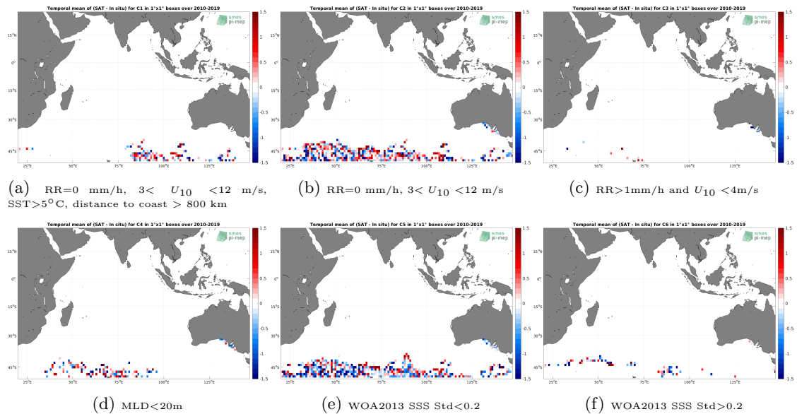
Figure 12: Temporal mean gridded over spatial boxes of size 1^{\circ}\times 1^{\circ} of \Delta\text{SSS} (SMOS SSS L2Q v331 - With FLAG (CMEMS-CATDS-CPDC) - Marine mammals) for 6 different subdatasets corresponding to:RR=0 mm/h, 3 < U_{10} < 12 m/s, SST >5^{\circ}\text{C} , distance to coast > 800 km (a), RR=0 mm/h, 3 < U_{10} < 12 m/s (b), RR >1 mm/h and U_{10} < 4 m/s (c),MLD <20 m (d),WOA2013 SSS Std <0.2 (e),WOA2013 SSS Std >0.2 (f).
