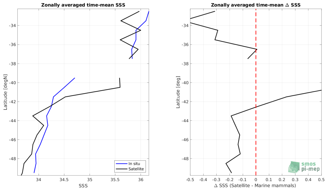
Figure 8: Left panel: Zonal mean SSS from SMOS SSS L2Q v331 - With FLAG (CMEMS-CATDS-CPDC) satellite product (black) and from Marine mammals (blue). Right panel: Zonal mean of \Delta SSS (Satellite - Marine mammals) for all the collected Pi-MEP match-up pairs estimated over the full satellite product period.
