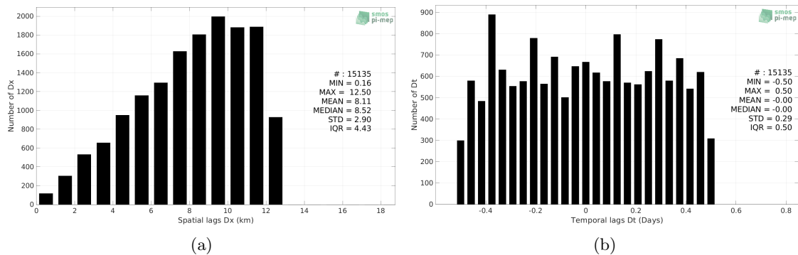
Figure 5: Histograms of the spatial (a) and temporal (b) lags between the location/time of the Marine mammals measurement and the date of the corresponding SMOS SSS L2Q v331 - With FLAG (CMEMS-CATDS-CPDC) SSS pixel.
