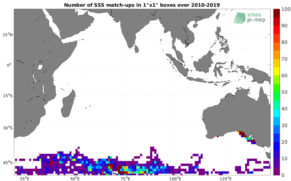
Figure 4: Number of SSS match-ups between Marine mammals SSS and the SMOS SSS L2Q v331 - With FLAG (CMEMS-CATDS-CPDC) SSS product for the Indian Ocean Pi-MEP region over 1^\circ \times 1^\circ boxes and for the full satellite product period.
