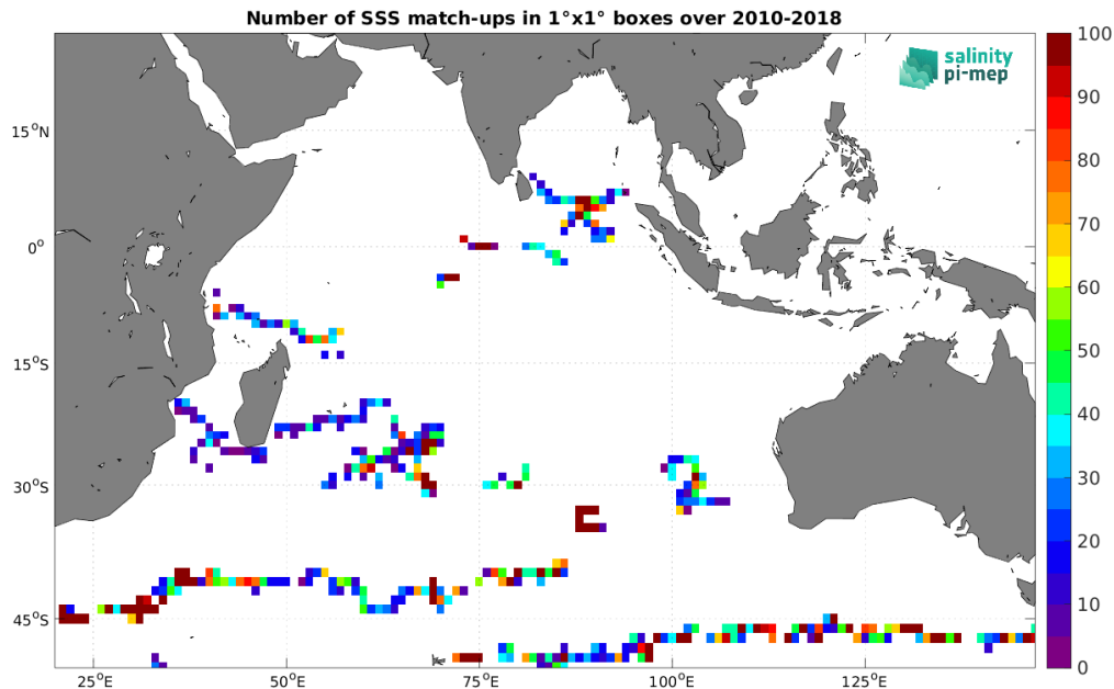
Figure 4: Number of SSS match-ups between Surface drifters SSS and the SMOS SSS L2Q v331 - With FLAG (CMEMS-CATDS-CPDC) SSS product for the Indian Ocean Pi-MEP region over 1^\circ \times 1^\circ boxes and for the full satellite product period.
