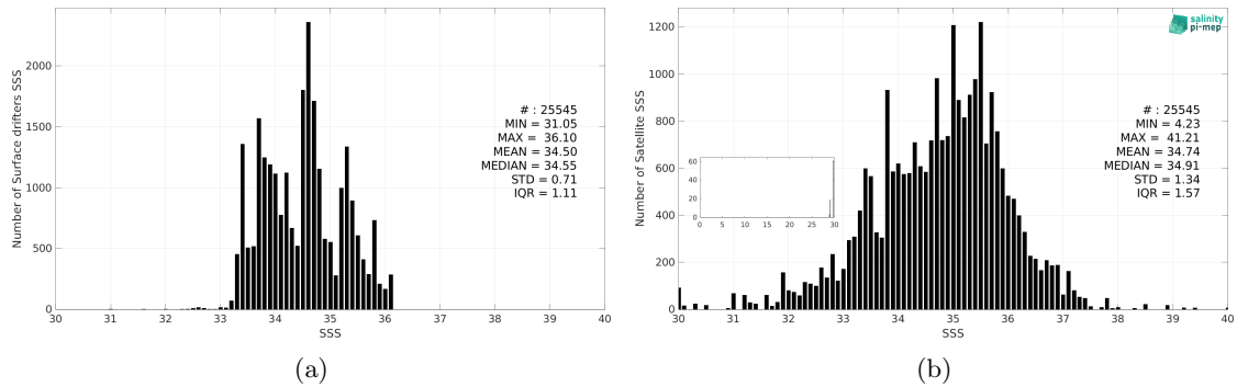
Figure 3: Histograms of SSS from Surface drifters (a) and SMOS SSS L2Q v331 - With FLAG (CMEMS-CATDS-CPDC) (b) considering all match-up pairs per bins of 0.1 over the Indian Ocean Pi-MEP region and for the full satellite product period.
