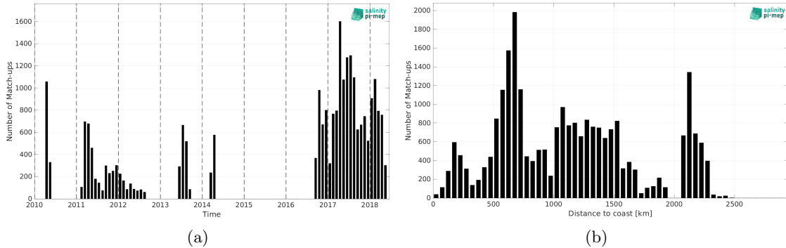
Figure 2: Number of match-ups between Surface drifters and SMOS SSS L2Q v331 - With FLAG (CMEMS-CATDS-CPDC) SSS as a function of time (a) and as function of the distance to coast (b) over the Indian Ocean Pi-MEP region and for the full satellite product period.
