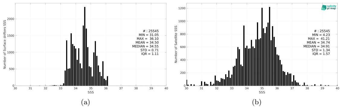
Figure 2: Histograms of SSS from Surface drifters (a) and SMOS SSS L2Q v331 - With FLAG (CMEMS-CATDS-CPDC) (b) considering all match-up pairs per bins of 0.1 over the Indian Ocean Pi-MEP region and for the full satellite product period.
