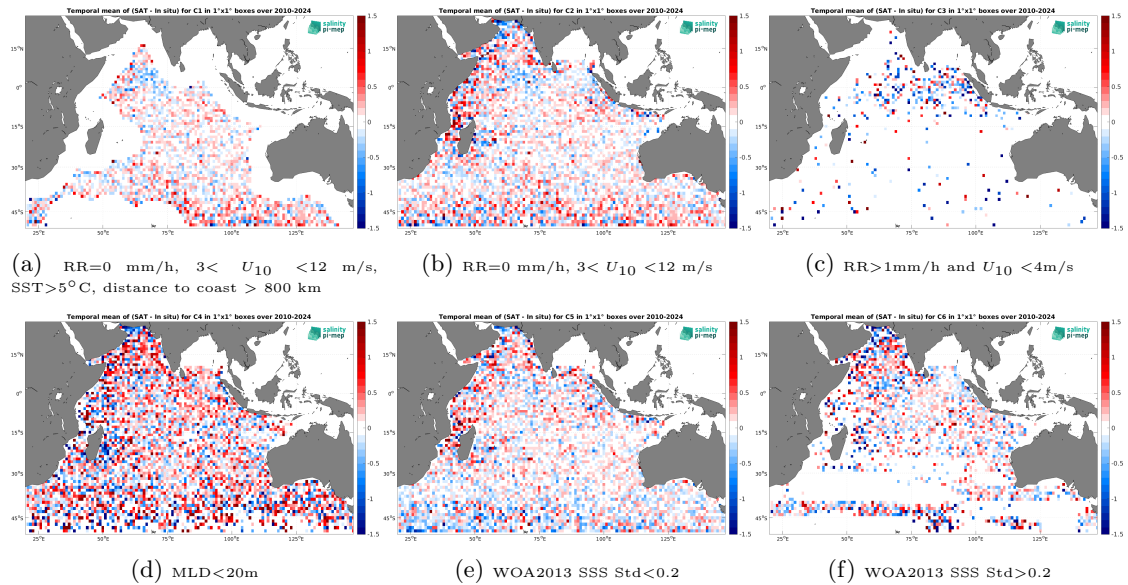
Figure 14: Temporal mean gridded over spatial boxes of size 1^\circ \times 1^\circ of \Delta SSS (SMOS SSS L2Q v331 - With FLAG (CMEMS-CATDS-CPDC) - Argo) for 6 different subdatasets corresponding to:RR=0 mm/h, 3 < U_{10} < 12 m/s, SST >5^\circ C, distance to coast > 800 km (a), RR=0 mm/h, 3 < U_{10} < 12 m/s (b), RR >1 mm/h and U_{10} < 4 m/s (c),MLD <20 m (d),WOA2013 SSS Std <0.2 (e),WOA2013 SSS Std >0.2 (f).
