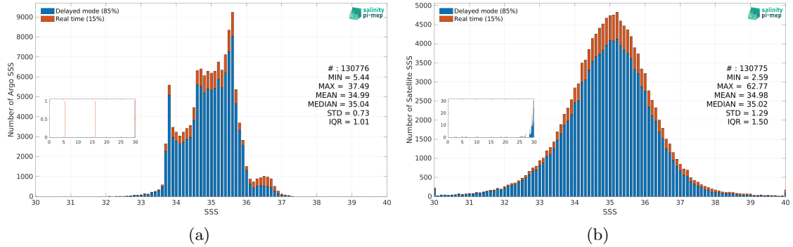
Figure 3: Histograms of SSS from Argo (a) and SMOS SSS L2Q v331 - With FLAG (CMEMS-CATDS-CPDC) (b) considering all match-up pairs per bins of 0.1 over the Indian Ocean Pi-MEP region and for the full satellite product period.
