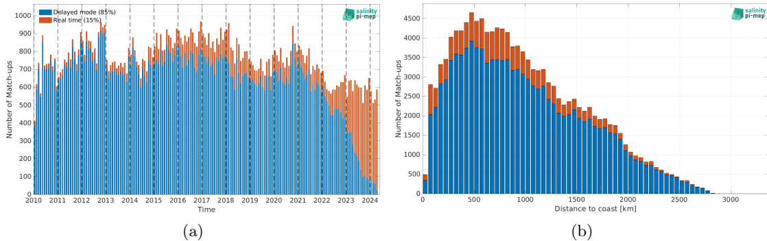
Figure 2: Number of match-ups between Argo and SMOS SSS L2Q v331 - With FLAG (CMEMS-CATDS-CPDC) SSS as a function of time (a) and as function of the distance to coast (b) over the Indian Ocean Pi-MEP region and for the full satellite product period.
