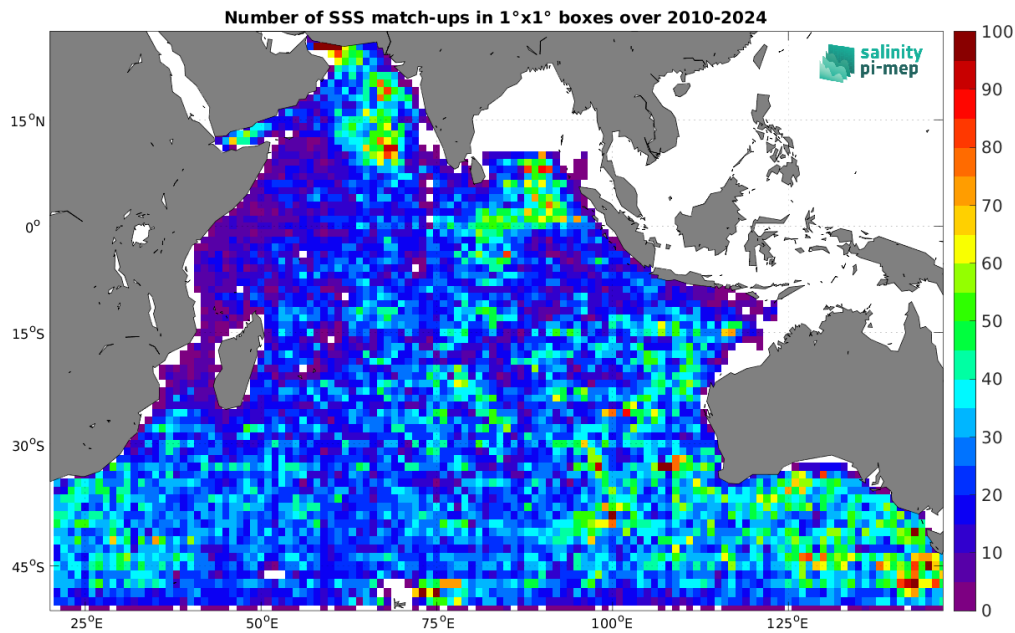
Figure 5: Number of SSS match-ups between Argo SSS and the SMOS SSS L2Q v331 - With FLAG (CMEMS-CATDS-CPDC) SSS product for the Indian Ocean Pi-MEP region over 1^\circ \times 1^\circ boxes and for the full satellite product period.
