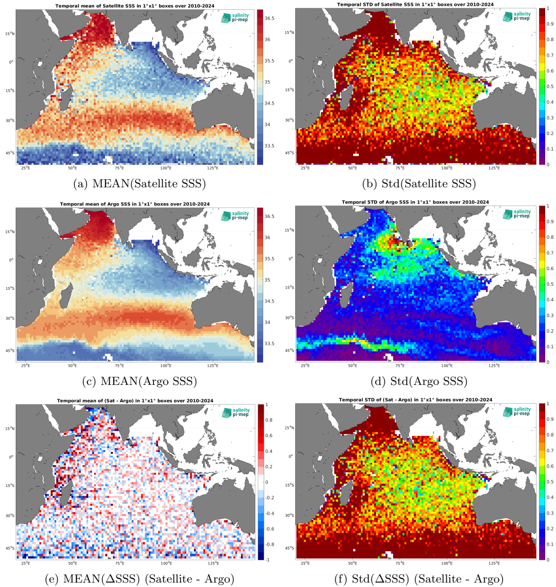
Figure 7: Temporal mean (left) and Std (right) of SSS from SMOS SSS L2Q v331 - With FLAG (CMEMS-CATDS-CPDC) (top), Argo (middle), and of \Delta SSS (Satellite - Argo). Only match-up pairs are used to generate these maps.
