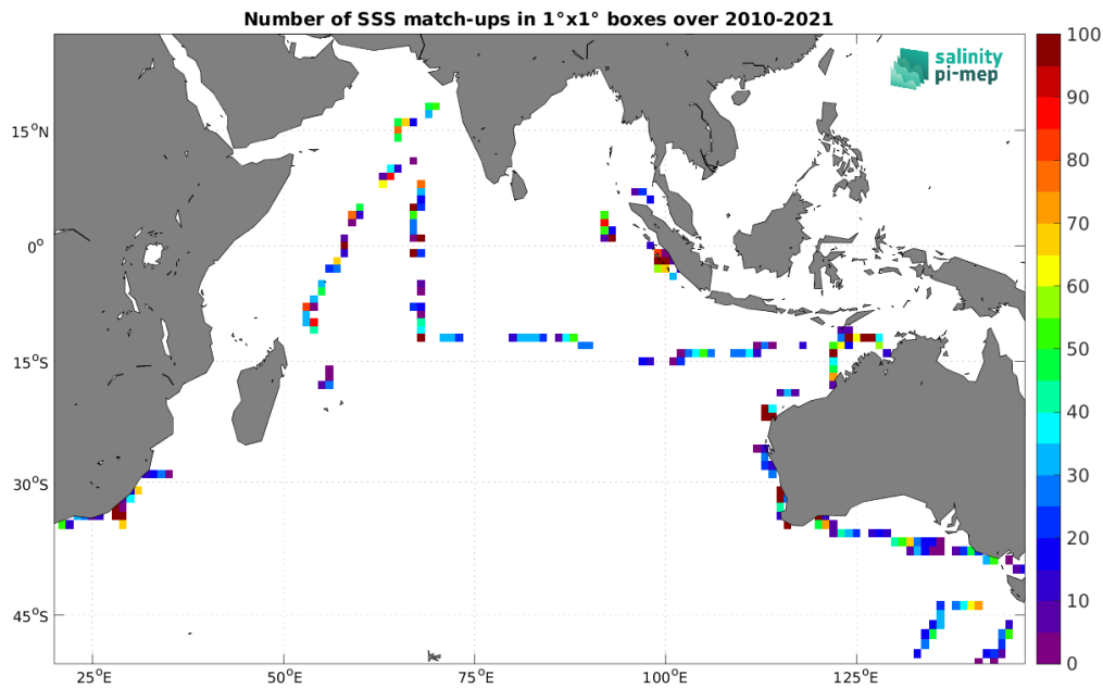
Figure 5: Number of SSS match-ups between TSG (SAMOS) SSS and the SMOS SSS L2Q v331 - No FLAG (CMEMS-CATDS-CPDC) SSS product for the Indian Ocean Pi-MEP region over 1^\circ \times 1^\circ boxes and for the full satellite product period.
