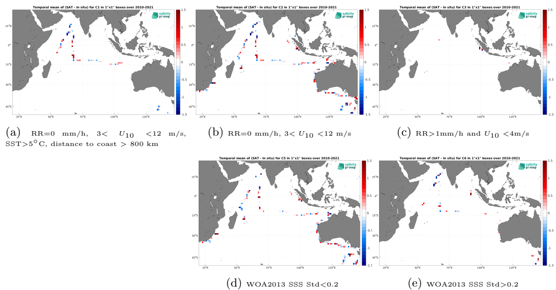
Figure 14: Temporal mean gridded over spatial boxes of size 1^\circ \times 1^\circ of \Delta SSS (SMOS SSS L2Q v331 - No FLAG (CMEMS-CATDS-CPDC) - TSG (SAMOS)) for 5 different subdatasets corresponding to:RR=0 mm/h, 3 < U_{10} < 12 m/s, SST >5^\circ C, distance to coast > 800 km (a), RR=0 mm/h, 3 < U_{10} < 12 m/s (b), RR >1 mm/h and U_{10} < 4 m/s (c), WOA2013 SSS Std <0.2 (d), WOA2013 SSS Std >0.2 (e).
