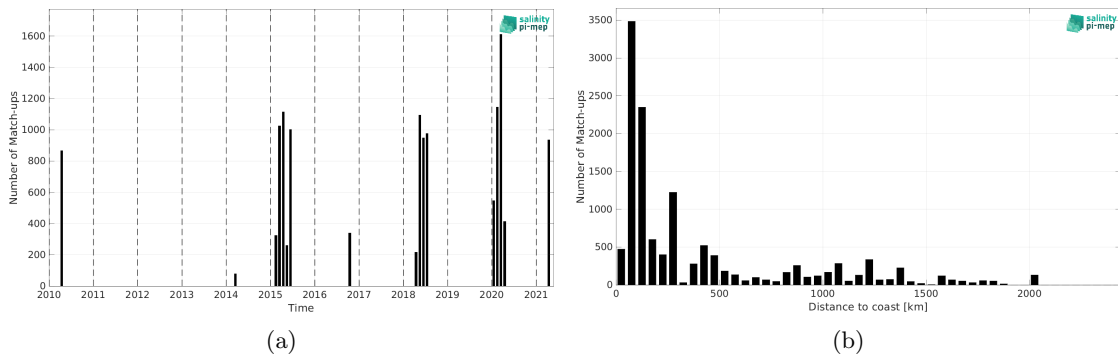
Figure 2: Number of match-ups between TSG (SAMOS) and SMOS SSS L2Q v331 - No FLAG (CMEMS-CATDS-CPDC) SSS as a function of time (a) and as function of the distance to coast (b) over the Indian Ocean Pi-MEP region and for the full satellite product period.
