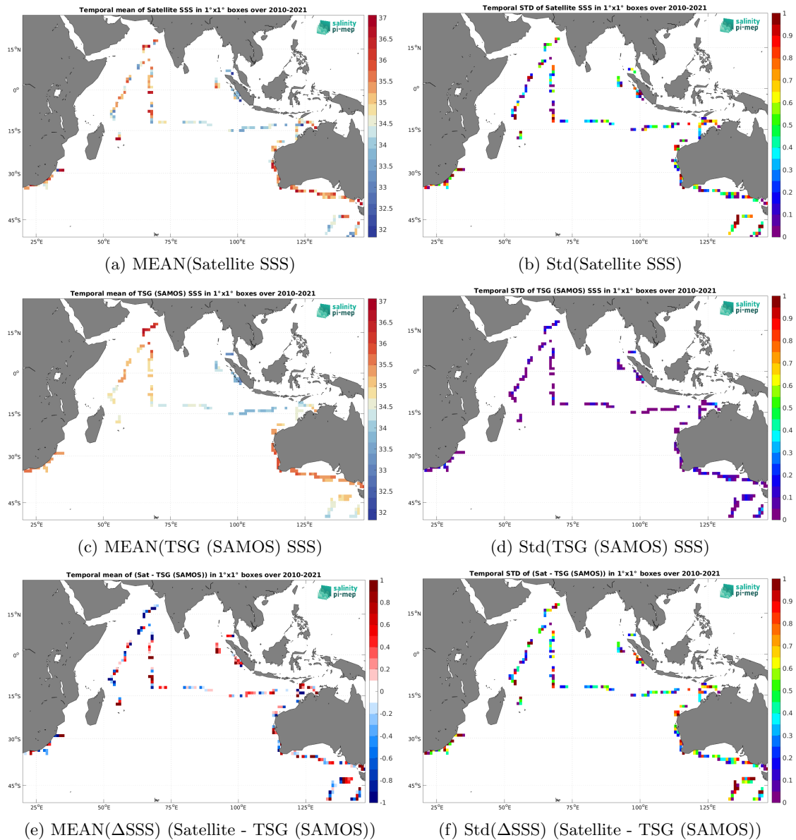
Figure 7: Temporal mean (left) and Std (right) of SSS from SMOS SSS L2Q v331 - No FLAG (CMEMS-CATDS-CPDC) (top), TSG (SAMOS) (middle), and of \Delta SSS (Satellite - TSG (SAMOS)). Only match-up pairs are used to generate these maps.
