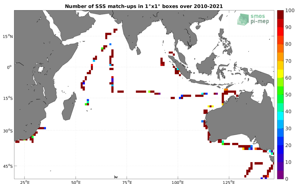
Figure 4: Number of SSS match-ups between TSG (SAMOS) SSS and the SMOS SSS L2Q v331 - No FLAG (CMEMS-CATDS-CPDC) SSS product for the Indian Ocean Pi-MEP region over 1^\circ \times 1^\circ boxes and for the full satellite product period.
