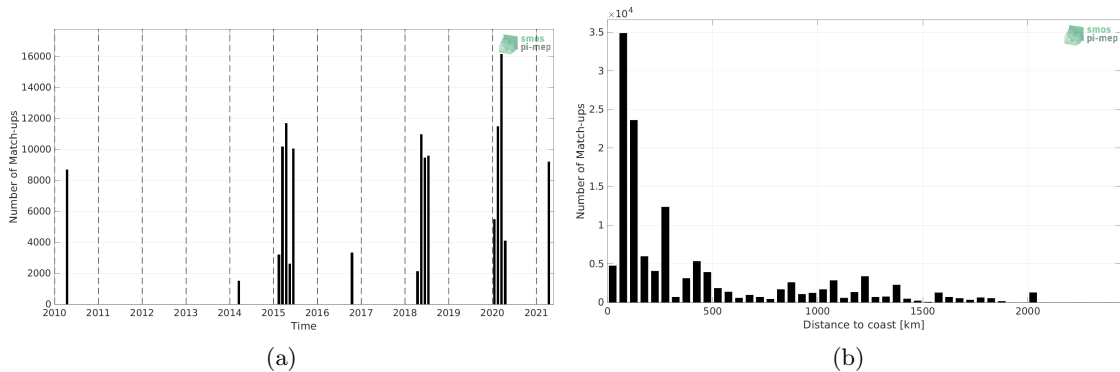
Figure 1: Number of match-ups between TSG (SAMOS) and SMOS SSS L2Q v331 - No FLAG (CMEMS-CATDS-CPDC) SSS as a function of time (a) and as function of the distance to coast (b) over the Indian Ocean Pi-MEP region and for the full satellite product period.
