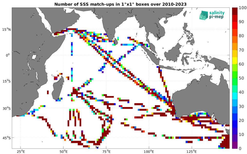
Figure 5: Number of SSS match-ups between TSG (LEGOS-DM) SSS and the SMOS SSS L2Q v331 - No FLAG (CMEMS-CATDS-CPDC) SSS product for the Indian Ocean Pi-MEP region over 1^\circ \times 1^\circ boxes and for the full satellite product period.
