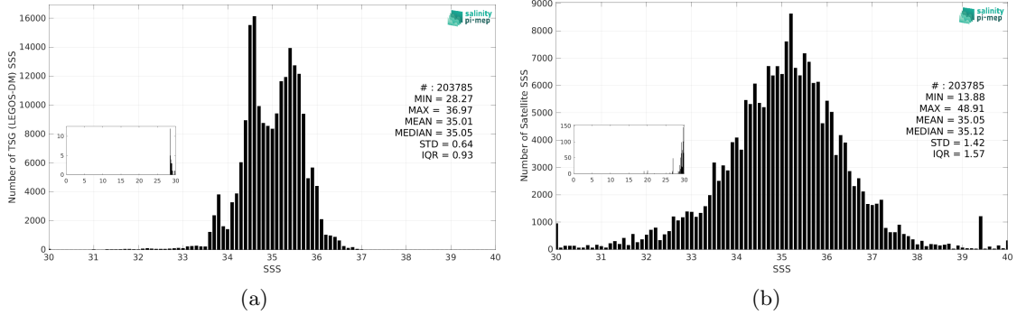
Figure 3: Histograms of SSS from TSG (LEGOS-DM) (a) and SMOS SSS L2Q v331 - No FLAG (CMEMS-CATDS-CPDC) (b) considering all match-up pairs per bins of 0.1 over the Indian Ocean Pi-MEP region and for the full satellite product period.
