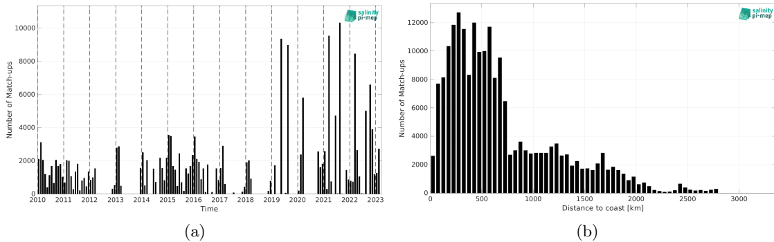
Figure 2: Number of match-ups between TSG (LEGOS-DM) and SMOS SSS L2Q v331 - No FLAG (CMEMS-CATDS-CPDC) SSS as a function of time (a) and as function of the distance to coast (b) over the Indian Ocean Pi-MEP region and for the full satellite product period.
