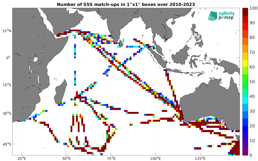
Figure 4: Number of SSS match-ups between TSG (LEGOS-DM) SSS and the SMOS SSS L2Q v331 - No FLAG (CMEMS-CATDS-CPDC) SSS product for the Indian Ocean Pi-MEP region over 1^\circ \times 1^\circ boxes and for the full satellite product period.
