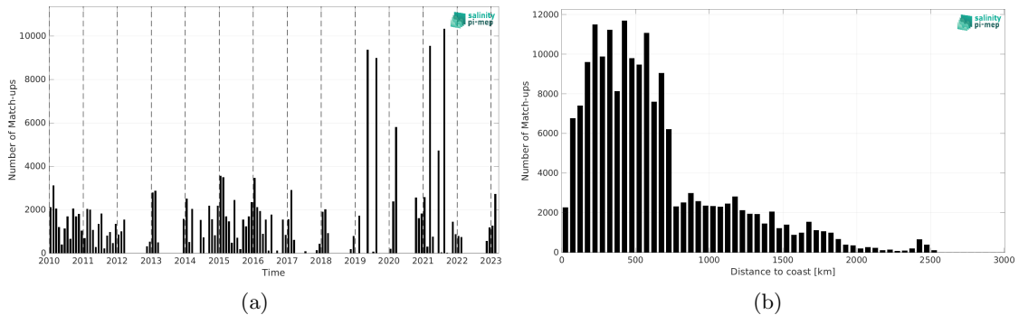
Figure 1: Number of match-ups between TSG (LEGOS-DM) and SMOS SSS L2Q v331 - No FLAG (CMEMS-CATDS-CPDC) SSS as a function of time (a) and as function of the distance to coast (b) over the Indian Ocean Pi-MEP region and for the full satellite product period.
