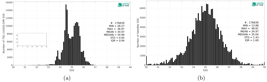
Figure 2: Histograms of SSS from TSG (LEGOS-DM) (a) and SMOS SSS L2Q v331 - No FLAG (CMEMS-CATDS-CPDC) (b) considering all match-up pairs per bins of 0.1 over the Indian Ocean Pi-MEP region and for the full satellite product period.
