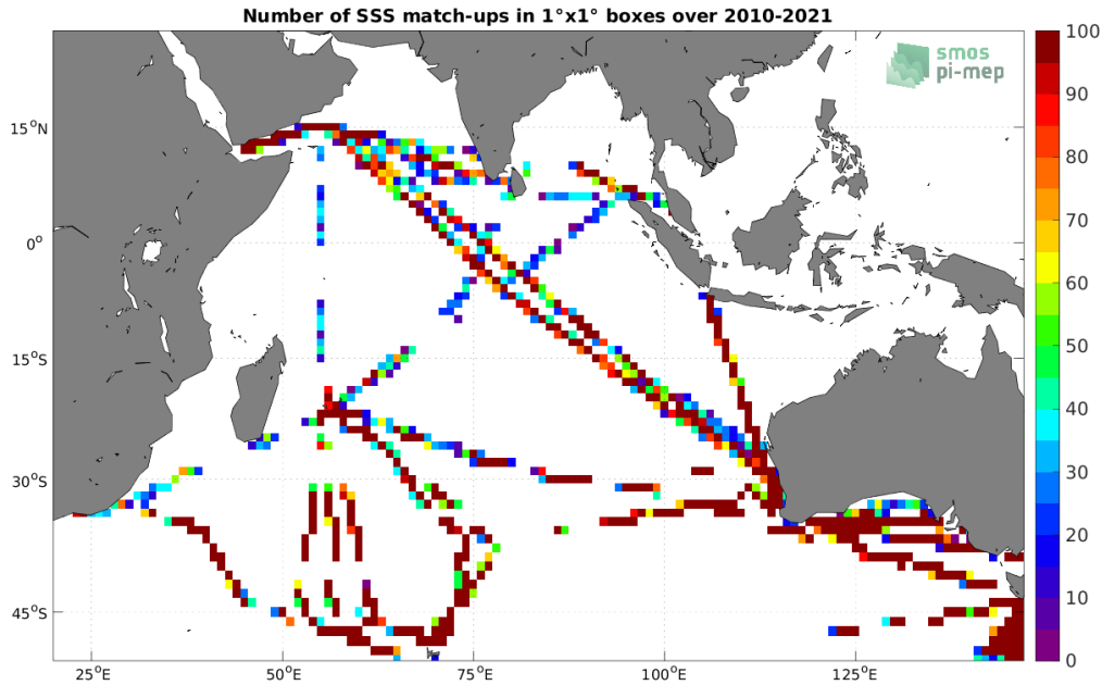
Figure 4: Number of SSS match-ups between TSG (LEGOS-DM) SSS and the SMOS SSS L2Q v331 - No FLAG (CMEMS-CATDS-CPDC) SSS product for the Indian Ocean Pi-MEP region over 1^\circ \times 1^\circ boxes and for the full satellite product period.
